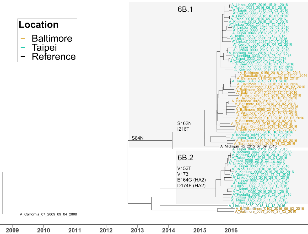
Figure 1. Phylogenetic tree of HA gene sequences from influenza H1N1pdm viruses obtained in the 2015-16 season. 6B.1 and 6B.2 clades with specific substitutions defining major branches indicated. Tips are colored by location of sample collection.
