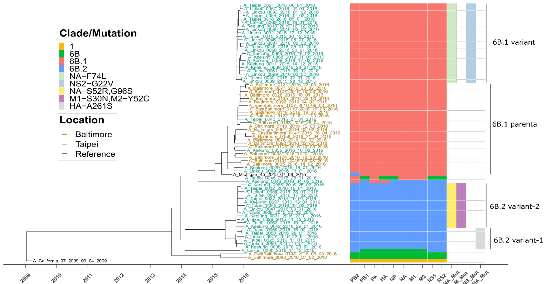
Figure 2. Phylogenetic tree of concatenated H1N1pdm segments with a schematic representation of four genetic subgroups and the mutations that define each.
