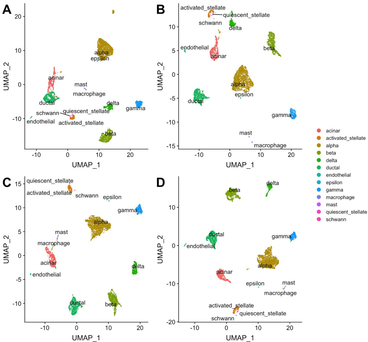
Figure S11: UMAP plots of two pancreatic datasets - CelSeq2 and SmartSeq2: integration results in “all cell types” experiment. Datasets are colored by cell types. A) BATMAN; B) Seurat V3.0; C) MNNcorrect; D) Scanorama.
