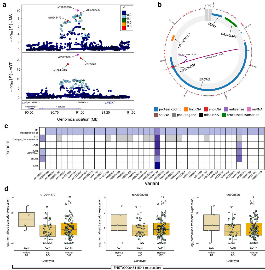
Figure 4: Fine-mapping of the BACH2 locus in CD4^+ T-cells. a , The locuszoom plot of the BACH2 locus using eQTL and MS data with 500kb flanking region surrounding the sentinel SNP rs72928038. Pairwise LD ( r^2 ) was calculated using BLUEPRINT data. The rs72928038 is an intronic variant of BACH2 and also known to be a risk allele (A) for MS 44 and T1D 41 . The locus was strongly colocalised ( PP_{coloc} \geq 0.98 ) between IMDs (MS and T1D) and multiple QTLs (i.e., eQTL, psiQTL, hQTL(H3K27ac) and mQTL) in naive T-cells. b , The sentinel variant, rs72928038, resides near the Transcriptional Start Site (TSS) of BACH2 . A significant chromatin interaction between rs72928038 and promoter of the BACH2 (Chicago score of 9.28) was observed in naive CD4^+ T-cell using PChIP data 53 , which shows a strong regulatory effect. The figure was generated by using ChIP web server 54 . c , Heatmap shows posterior probability of the fine-mapped variants ( PP_{fm} ) in the respective credible sets (colour intensity: PP_{fm\_smallest} - light blue to PP_{fm\_largest} - deep blue). White colour indicates the variants were not part of the respective credible sets. Due to lack of variant density in T1D summary statistics, many variants were not tested for fine-mapping analysis (grey). The locus could not be fine-mapped confidently with MS summary statistics, yielded a credible set of 40 variants (rs72928038 being the top variant; PP_{fm} = 0.3 ), whereas a single variant (rs72928038; PP_{fm} = 0.98 ) credible set was achieved by using eQTL data. The rs72928038 appeared to be the most likely causal variant in all
