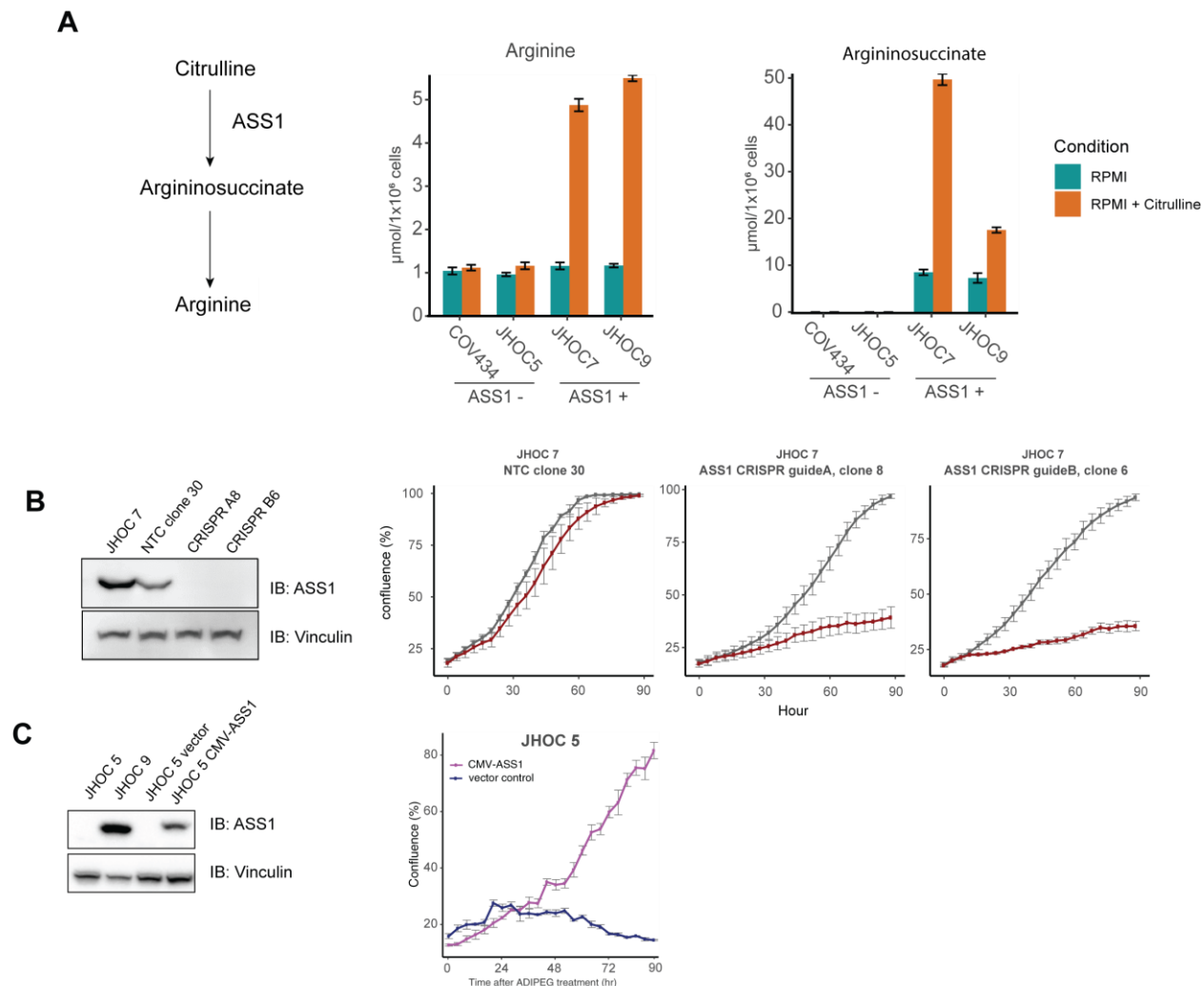
Figure 4. ASS1 is required for survival in arginine deplete conditions and its deficiency disrupts urea cycle function. A , Argininosuccinate and arginine intracellular measurements in ASS1-deficient cells (JHOC 5 and COV434), compared to ASS1- proficient cells (JHOC 7 and JHOC 9). B , western blot showing the knockout efficiency of two CRISPR ASS1 knockout clones in a JHOC 7 background (A8: clone 8 using guide A, and B6: clone 6 using guide B, NTC30: empty vector negative control). and the specificity of ADI-PEG20 was confirmed in the ASS1 knockout clones A8 and B6. C , Western blot showing the stable over-expression of ASS1 in JHOC5, rescuing its growth when treated with 0.63 \mu g/mL of ADI-PEG20. All p-values were generated from student t-test. Error bars represent standard error of mean.
