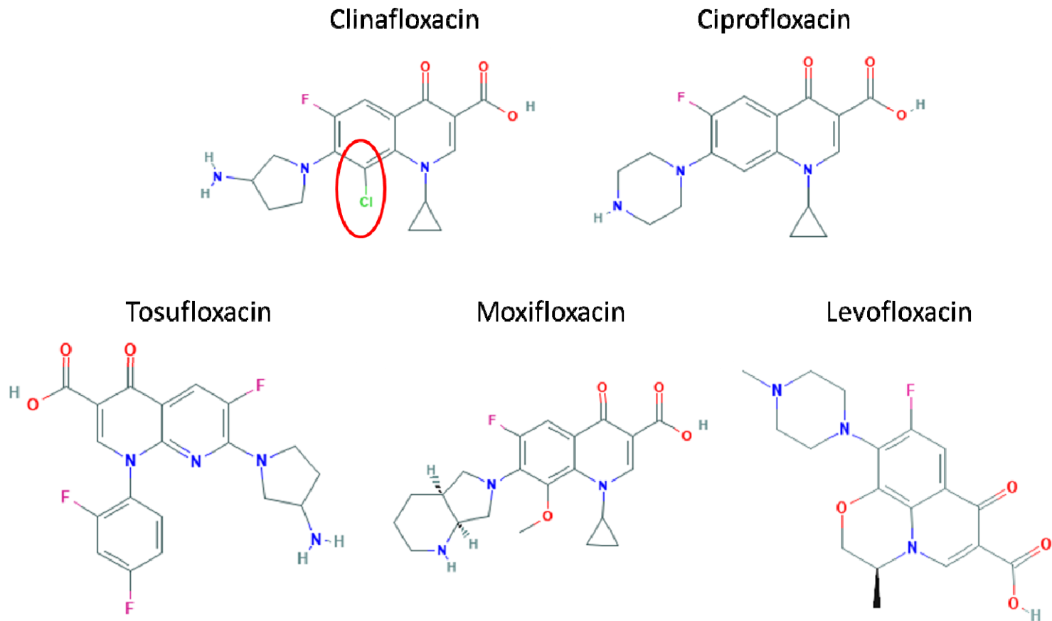
Figure 6. Chemical structures of the fluoroquinolones tested. The chloride group (circled) is unique to clinafloxacin.
