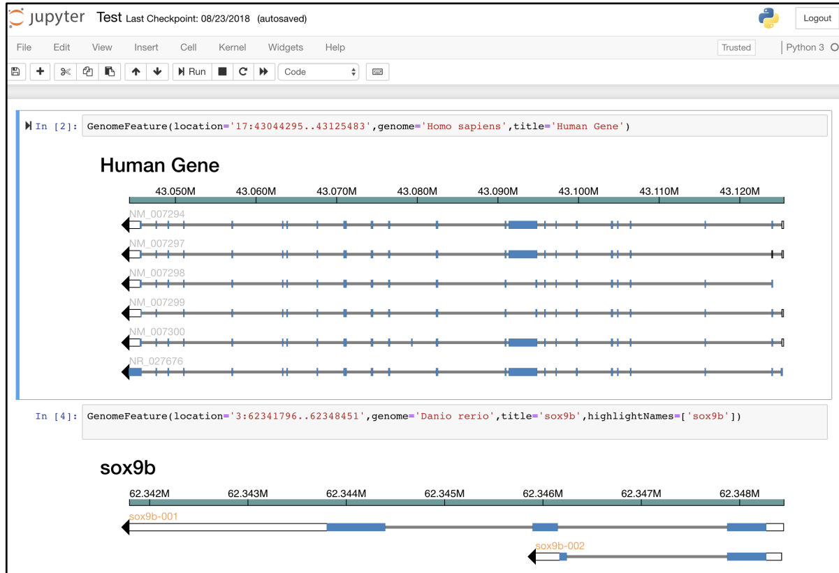
Figure 5. Three demonstrations of the Genome Feature Component npm widget ( https://www.npmjs.com/package/genomefeaturecomponent ) show examples that leverage Apollo's web services by consuming snippets of data for particular regions. A) The Alliance for Genome Resources web page ( https://www.alliancegenome.org/gene/HGNC:1100 ) visualizes the Human BRCA1 gene. B) the Monarch Initiative ( https://monarchinitiative.org/ ) web page visualizes the human IL2 gene. C) We embed the npm widget within a Jupyter Notebook widget to be called directly from a Python command-line script.
