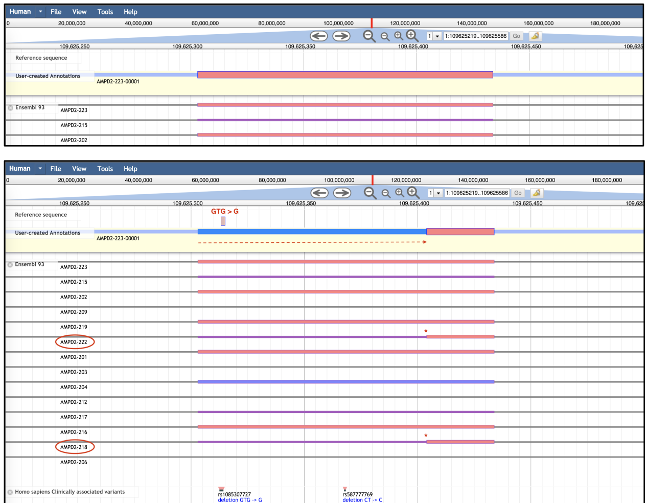
Figure 3. Example of variant annotation in Apollo. A) AMPD2-223, an isoform of gene AMPD2 as seen from the Evidence Area (truncated for space). From AMPD2-223, an isoform is dragged into the Editing Area. B) The deletion variant rs1085307727, from the 'Homo sapiens Clinically associated variants' track, overlaps with AMPD2-223-00001. Creating a corresponding deletion in the Editing Area of the Sequence Track allows visualization of the effect of the variant on transcript AMPD2-223-00001. Here, the transcription start site has moved further downstream, as indicated by the red dashed line. In this case, the altered form of the transcript recapitulates other alternate isoforms for this gene (AMDP2-218 and AMPD2-222), which are circled and starred for clarity.
