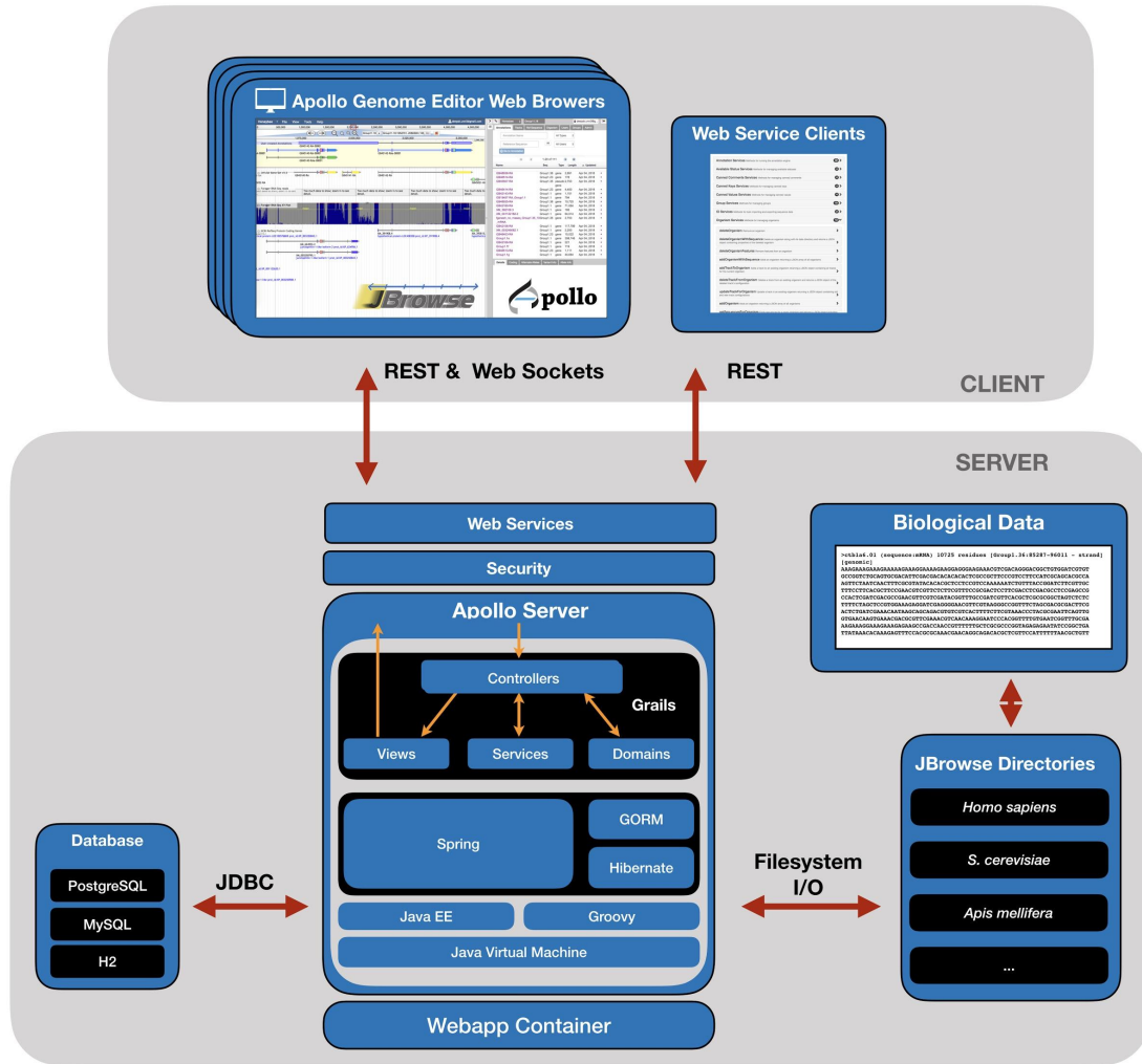
Figure 2: Apollo's client-server architecture. The server is built over the Grails framework using a relational database backend (RDBMS), for example PostgreSQL, MySQL or H2. Genomic evidence is provided by pointing to existing JBrowse directories that contain processed biological data. The Apollo Genome Editor and Web Services clients communicate with the server via REST and WebSockets.
