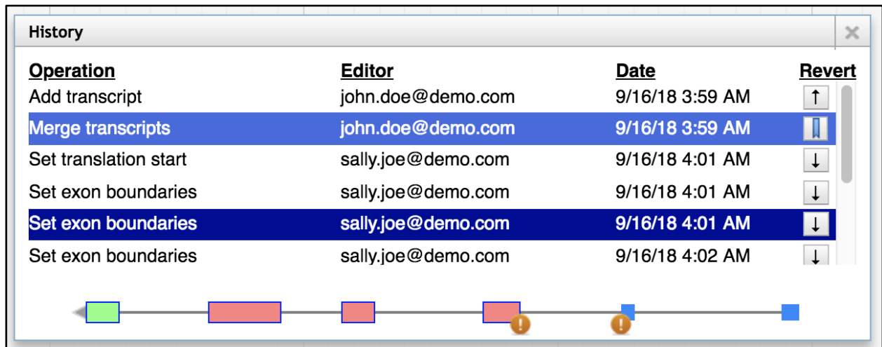
Figure 4. The history navigator allows visual navigation of genomic edits as well as the ability to return to previous versions. The current version is indicated with a bookmark icon (in the Revert column). Users can select any version from the history, and make edits starting from that version if desired. The orange circles with an exclamation point indicate non-canonical splice sites.
