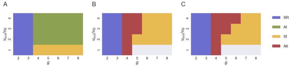
Figure 2. Diagrams of the different regimes for each version of the Brunel network ((A), (B) and (C) corresponding to versions 1, 2, and 3 of the network, respectively) in the parameter space (\nu_{\text{ext}}/\nu_{\theta}, g) . The white areas indicate where no neurons fired and no data is available.
