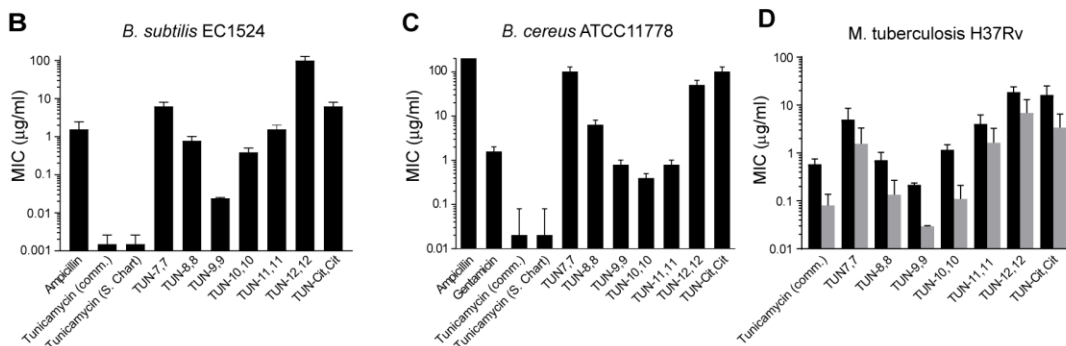
Figure 5. Design, semi-synthetic synthesis and antibacterial effects of TUN-X,X analogues.
