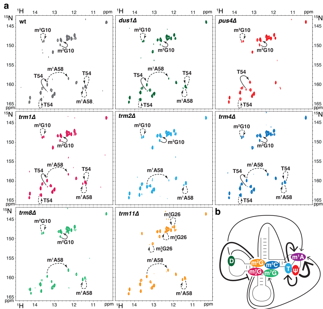
Figure 5 Complex modification circuits in yeast tRNA Phe .
