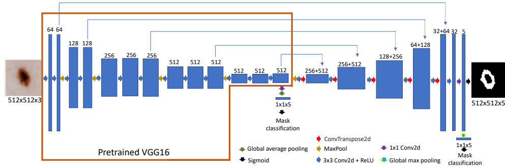
Figure 1: Network structure using in U-Net based approach. The encoder part of the U-Net is replaced with a pretrained VGG16 network [Shvets et al., 2018]. We also add two classification heads to the network, where one is added to the middle layer with 1 \times 1 convolution and global average pooling layers and the other is added to the last layer with a global max pooling layer.
