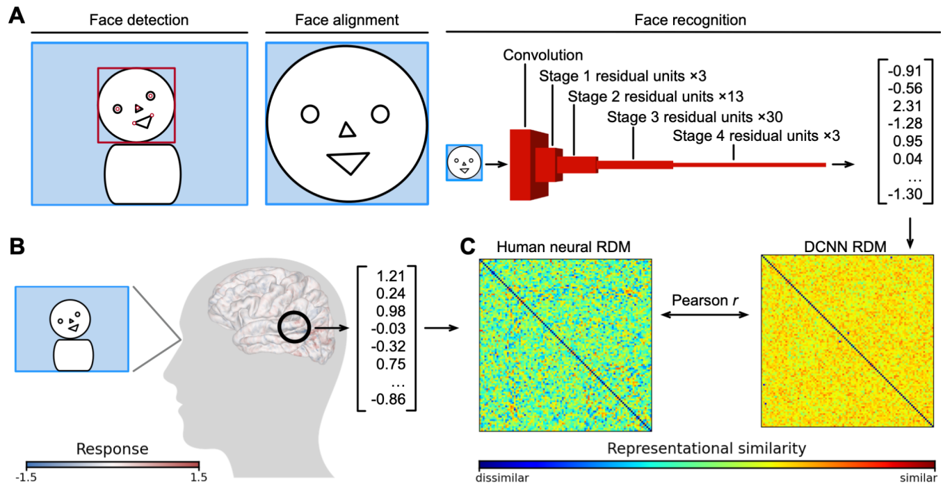
Figure 1. Schematic illustration of deep convolutional neural network (DCNN) and human neural representations of faces. A. The DCNN face recognition process comprised three steps. First, the face and its five key landmarks were automatically detected in each frame, and these landmarks were used to create the image of the aligned and cropped face. The cropped face image was then fed into the DCNN as input, and passed through convolutional layers, residual units, and fully-connected layers. The final output was a 512-dimensional embedding vector. Each video clip comprised 120 frames, and the corresponding 120 vectors were averaged to obtain an average embedding vector for each clip. Note that this illustrative example was based on the fully-connected layer of ArcFace. B. Human participants watched the face video clips in the fMRI scanner, and their brain responses were recorded. For each brain region (searchlight), the responses of multiple vertices in the region formed a spatial pattern, and the resulting pattern vector was considered the neural representation of the face clip for that brain region. C. For each brain region, we computed the dissimilarities between the pattern vectors of the 707 face clips, which formed a 707 \times 707 representational dissimilarity matrix (RDM). Similarly, we created a DCNN RDM based on dissimilarities between the 707 embedding vectors. We used the Pearson correlation between the two RDMs to assess the similarity between DCNN and neural representations. Note that this figure is illustrative and not based on real data nor actual face clips used in the experiment.
