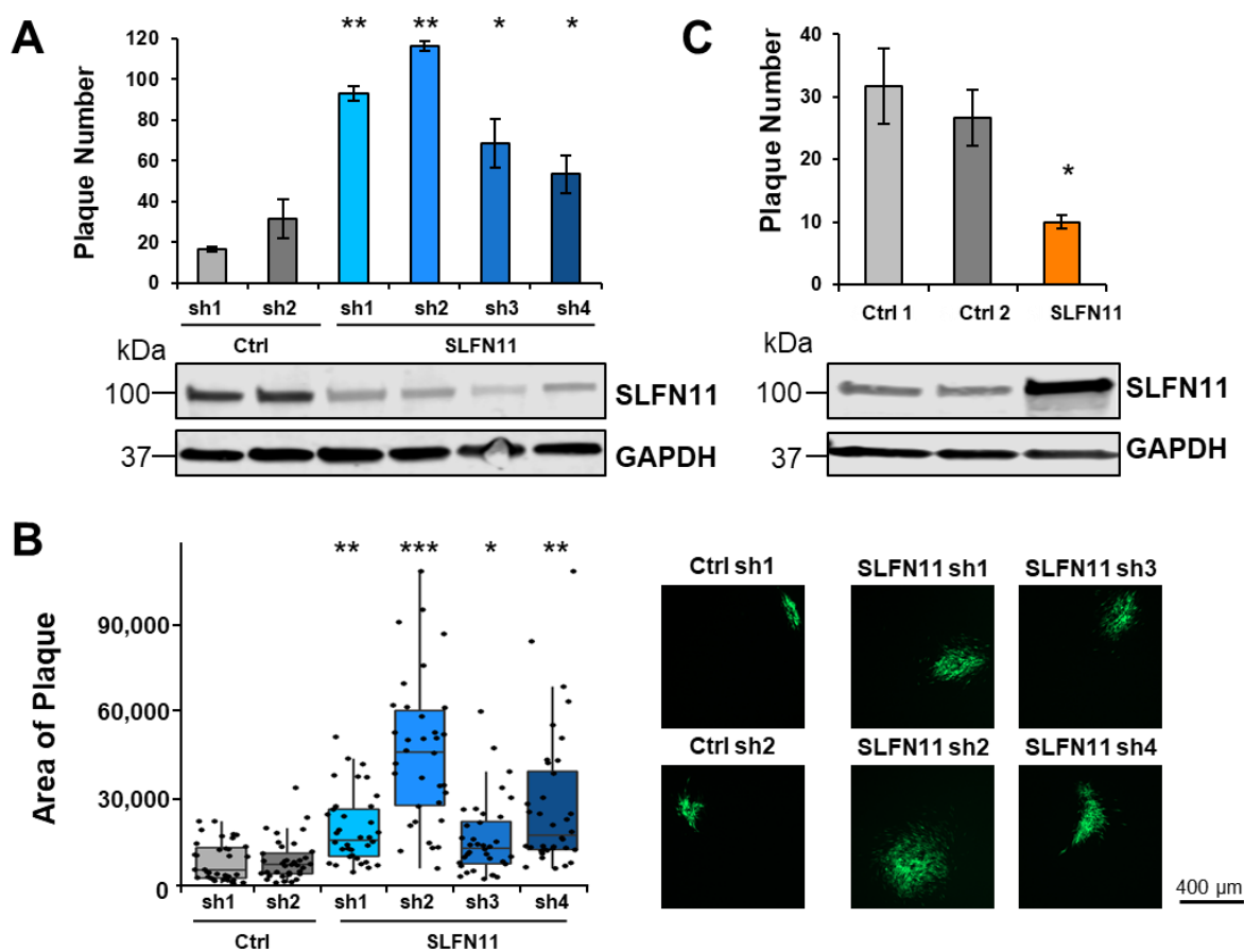
Figure 4. SLFN11 restricts HCMV infection
