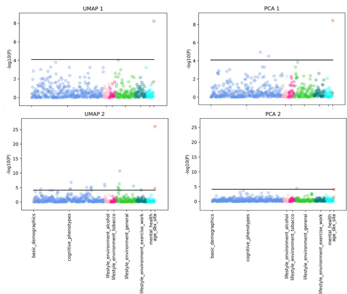
Figure 7: Manhattan plot of p-value of univariate correlation of non-imaging measures with UMAP of latent variables (left) and first two components of PCA (right) for faces-Shapes subtask. The black line is Bonferroni-corrected p-value threshold.
