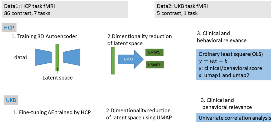
Figure 1: Method's overview
