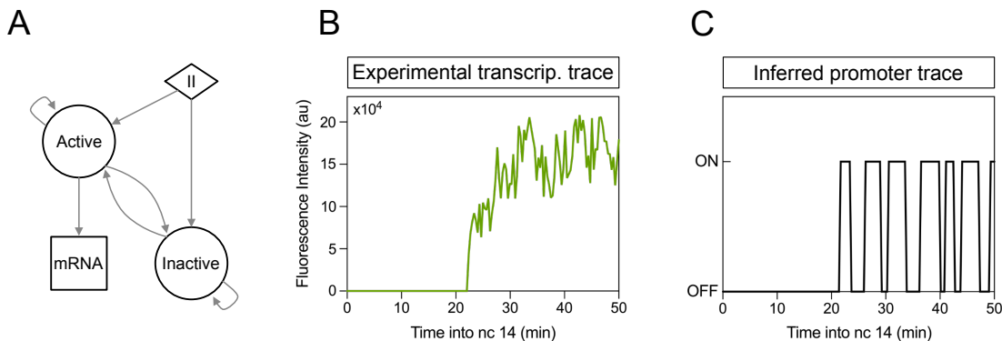
Figure 1: The model structure and basic principle behind burstInfer . A : Dynamic memory-adjusted hidden Markov model state diagram. At the beginning of the time sequence the promoter is in either the active or inactive state ( \pi ). Over the course of the time series the promoter switches stochastically between the active and inactive states according to the k_{\text{on}} and k_{\text{off}} burst parameters. While in the active state Pol II molecules are loaded onto the gene and mRNA transcripts are produced at a rate determined by the model emission parameter. B : Example MS2 fluorescence time series trace for a single nucleus in a Drosophila embryo showing nascent ush transcription. C : The promoter sequence inferred by the model corresponding to the fluorescent trace in B. These promoter traces can be used to generate single-cell parameters.
