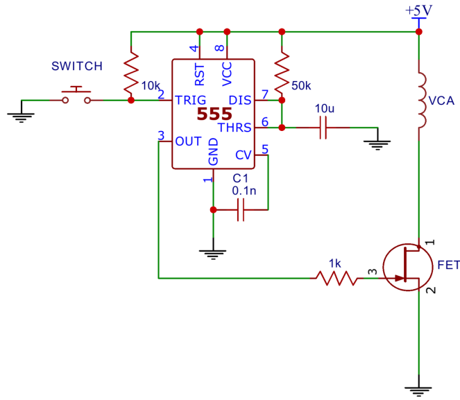
Figure 2. Dedicated mechanical apparatus.
