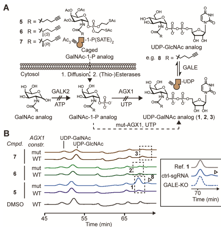
Fig 4: Substrate delivery to the cytosol of living cells. a , schematic of substrate delivery. Non-permissive steps are indicated by crossed arrows. The epimerase GALE interconverts UDP-GlcNAc and UDP-GalNAc. b , HPAEC-PAD traces of extracts from HEK293T cells stably expressing WT-AGX1 or mut-AGX1 and fed with the indicated compounds. Dashed boxes indicate retention times of standards in separate reference runs (Fig. S4B). The product of potential epimerization of 1 by GALE, compound 8 , is marked with an arrowhead. Data is of one experiment and was repeated for compound 5 in HEK293T cells transiently transfected with AGX1 constructs, as well as stably transfected K-562 cells (Fig. S4B and fig. S5). Insert: epimerization to 8 is
