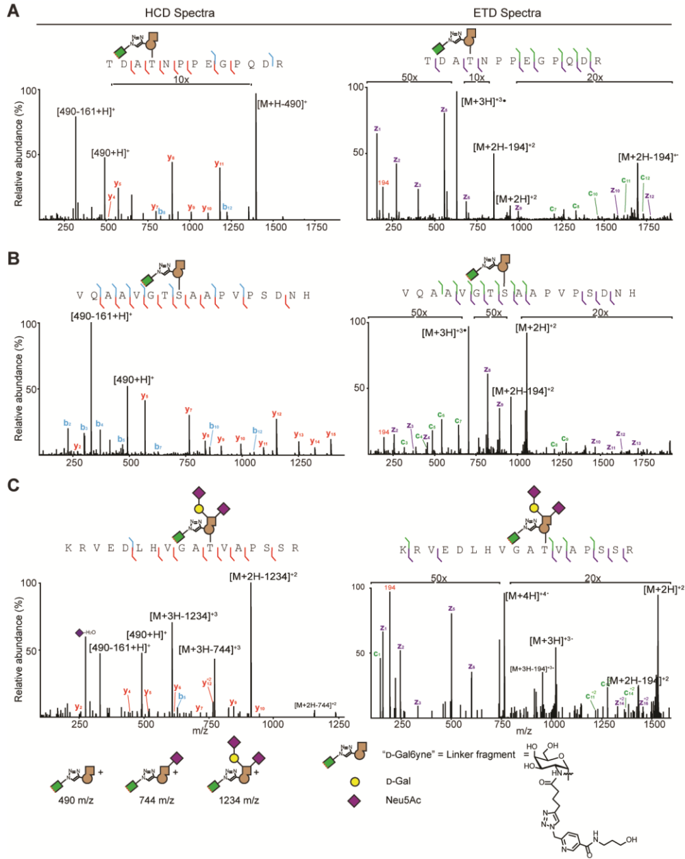
Fig. S9. Exemplary mass spectra from glycopeptides after modification by DM-T-2. HCD (mainly glycan fragmentation) and ETD (mainly peptide fragmentation) spectra are shown, and ions are annotated. A , glycosylation at Thr28 of STC2 as a newly-identified T-2-specific modification (63). B , confirmation of Ser308 as a T-2-specific modification of ApoE. C , extension of chemically tagged GalNAc by elaborating glycosyltransferases on T39 of SERPIN5A. Legend depicts tentative structural assignments of oxonium ions. Loss of 161 m/z in HCD and 194 m/z peak in ETD likely depicts fragment masses of the triazole-based linker.
