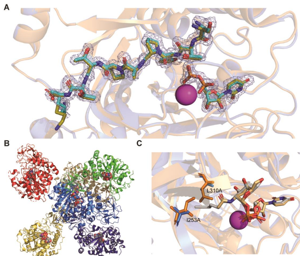
Fig. S1. A , overlay of ligands bound in DM-T-2/EA2/UDP/Mn 2+ (ligands cyan) and a published crystal structure of WT-T-2/EA2/UDP/Mn 2+ (ligands olive, PDB 2FFU), with electron density (map rendered at 1 \sigma and carved at 1.6 Å) taken from the DM-T-2 co-crystal structure. Mn 2+ ions are colored in magenta and overlay completely. B , crystal structure of DM-T-2/1/Mn 2+ in the hexameric unit cell. UDP-GalNAc analog 1 is rendered in sphere representation. C , superposition of the active sites of WT-T-2 (PDB 4D0T, orange) with UDP-GalNAc (light brown) and DM-T-2 (blue) with UDP-GalNAc analog 1 (grey). Gatekeeper residues are rendered in stick representation. Mn 2+ ions are magenta and overlay completely.
