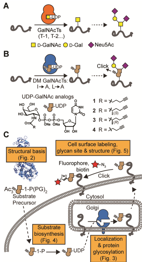
Fig. 1: GalNAcT bump-and-hole engineering. A , GalNAcTs initiate O-GalNAc glycosylation. B , Transfer of GalNAc to a Ser or Thr side chain is followed by downstream glycan elongation. C , the principle of bump-and-hole engineering. Engineered double mutant (DM) GalNAcTs are paired with UDP-GalNAc analogs 1-4 to chemically tag GalNAcT substrates that can be monitored by click chemistry. C , Overview of the steps taken in this study toward GalNAcT bump-and-hole engineering in the living cell. PG = Protecting group.
