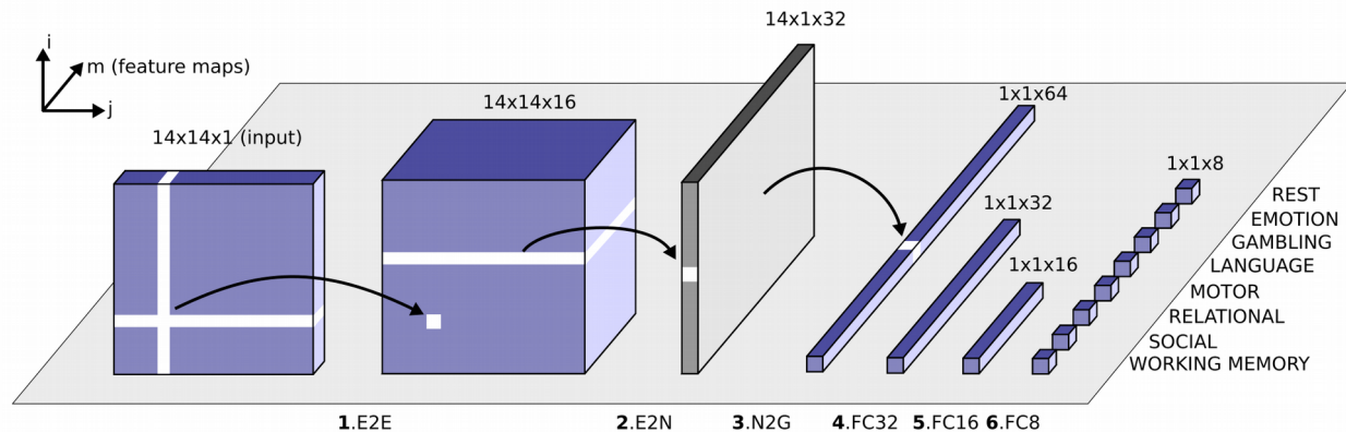
Figure 1: Schematic overview of the modified convolutional neural network architecture used to classify the eight different network configurations (seven tasks and one resting state; Kawahara et al., 2017). Each block represents the input/output of a numbered filter layer. The third dimension ( m ) represents the result of convolving the input with m different filters (feature maps). First, an interaction matrix composed of the interactions of 14 networks (based on synchrony or metastability) is entered as input. This is convolved with an edge-to-edge (1. E2E) filter which weights the edges associated with adjacent brain networks in topological space. The output from this layer is then convolved with an edge-to-node (2. E2N) filter which assigns each network a weighted sum of its edges. Next, a node-to-graph (3. N2G) layer outputs a single response based on all the weighted nodes. Finally, the number of features is reduced to eight output classifications through a series of fully connected (4/5/6. FC) layers.
