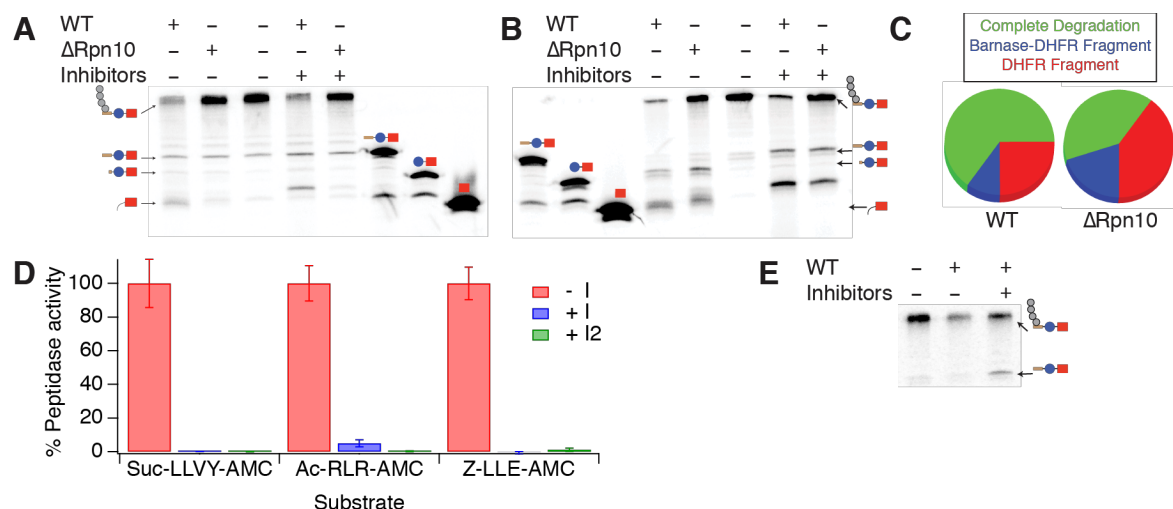
Figure 2. \Delta Rpn10 proteasome has a processivity defect. A, B ) Degradation of trace radiolabeled Keap1- ( A ) or Rsp5-ubiquitinated substrate ( B ) by 100 nM wild-type or \Delta Rpn10 proteasome (2 hours). Fragments containing either DHFR plus a small tail or Barnase-DHFR plus a small tail were identified relative to size standard control constructs (Neh2Dual-Barnase-DHFR, Barnase-DHFR and DHFR). Proteasome inhibitors (100 \mu M each MG-132, Bortezomib and 1,10-phenanthroline) were added as indicated. Based on quantification, less than 10% of the full-length Keap1-ubiquitinated protein was degraded by \Delta Rpn10 proteasome. Note that similar or greater levels of fragment were formed with \Delta Rpn10 and the Rsp5-ubiquitinated substrate despite a far lesser extent of degradation. C ) Quantification (based on two replicate experiments) of the relative frequency of complete versus partial degradation for wild-type versus \Delta Rpn10 proteasome with the Rsp5-ubiquitinated substrate. Protein that did not undergo degradation was ignored. D ) Peptidase activity in the absence (red) or presence of proteasome inhibitors as in B (blue; I) or with 100 \mu M epoxomicin replacing 1,10-phenanthroline (green; I2). The first cocktail reduces Suc-LLVY-AMC (chymotrypsin-like) activity to 0.1% ( p = 0.07 when comparing proteasome plus inhibitors to background reaction), reduces Ac-RLR-AMC (trypsin-like) activity to 5% of uninhibited rates ( p = 0.001 ), and eliminates Z-LLE-AMC (peptidyl glutamyl hydrolase-like) activity (at or below background rates). With the second cocktail, all rates are indistinguishable from background. Error bars are the SEM of 4 replicate assays. E ) Degradation of trace radiolabeled Rsp5-ubiquitinated substrate by 100 nM wild-type proteasome in the absence or presence of 100 \mu M each MG-132, Bortezomib, and epoxomicin. No NADPH was added to stabilize DHFR in this experiment.
