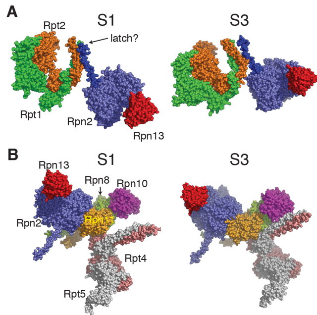
Figure 8. Conformational changes that could link ubiquitin binding to proteasomal activation. Left is S1 state (PDB IDs 5MP9 & 5MPD), right is S3 state (PDB ID 5MPB) A) Reorientation of Rpn13 (red) is correlated with movement of an Rpn2 (purple) helix (blue) to minimize contact with the Rpt1 (green)/Rpt2 (orange) coiled-coil. B) The Rpn8 (light green)/Rpn11 (light orange) heterodimer connects Rpn10 (magenta) and Rpn2. Rpn10 contacts the Rpt4 (salmon)/Rpt5 (grey) heterodimer in the S3 but not the S1 state.
