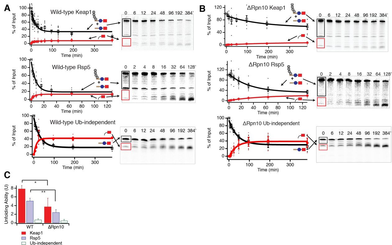
Figure 3. Unfolding abilities of wild-type versus \Delta Rpn10 proteasomes. A, B ) Degradation of trace radiolabeled Keap1- or Rsp5-ubiquitinated substrate or ubiquitin-independent substrate (yO44-Barnase-DHFR-His) with a destabilized barnase domain by 100 nM wild-type ( A ) or \Delta Rpn10 ( B ) proteasome. Black box shows region of the gel containing full-length protein with or without ubiquitination. Red box shows the region of the gel containing the DHFR fragment. The amounts of full-length protein (open squares) and DHFR fragment (red circles) are shown as a percentage of the ubiquitinated full-length substrate presented to the proteasome at the beginning of the reaction (or the full-length protein for the ubiquitin-independent substrate); the full-length protein is quantified as the sum of ubiquitinated and non-ubiquitinated full-length species so any deubiquitination is not misinterpreted as degradation. Dots are results from individual experiments, and error bars represent the SEM of 6-22 experiments. Curves are global fits to single exponentials. Sample gels are shown on the right. C ) Unfolding abilities (U) calculated from the curve fits shown in A and B . Error bars are the SEM propagated from curve fitting the collected data sets. * indicates p \leq 0.05 , ** indicates p \leq 0.01 relative to wild-type.
