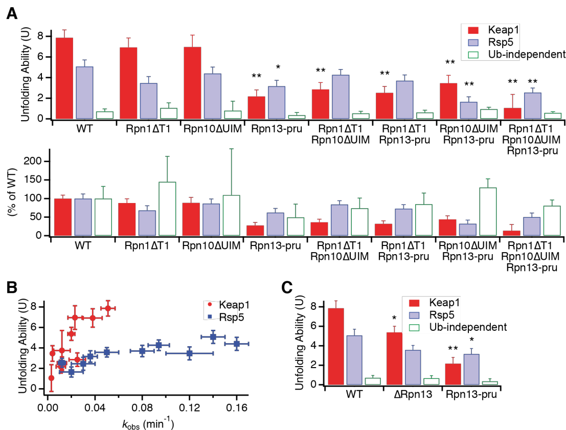
Figure 4. Ubiquitin receptor mutants have varied effects on proteasomal unfolding ability. A ) Top: Effect of point mutants in ubiquitin binding domains on proteasomal unfolding ability, as measured using Keap1 (red) or Rsp5 (blue) ubiquitinated substrates or a ubiquitin-independent substrate (green). Error bars are the SEM propagated from curve fitting 4-22 collected data sets. * indicates p \leq 0.05 , ** indicates p \leq 0.01 relative to wild-type. Bottom: unfolding abilities of mutants as normalized to wild-type proteasome. B ) Unfolding ability (From panel A above) versus observed rate constant for disappearance of full-length protein ( k_{obs} ) for Keap1 (red circles) and Rsp5 (blue squares) ubiquitinated substrates (from curve fits in Figure 3A and Figure S4 ). C ) Rpn13 deletion ( \Delta Rpn13) has a smaller effect on proteasomal unfolding ability than Rpn13 point mutations that prevent ubiquitin binding (Rpn13-pru). Error bars are the SEM propagated from curve fitting 4-22 collected data sets. * indicates p \leq 0.05 , ** indicates p \leq 0.01 relative to wild-type.
