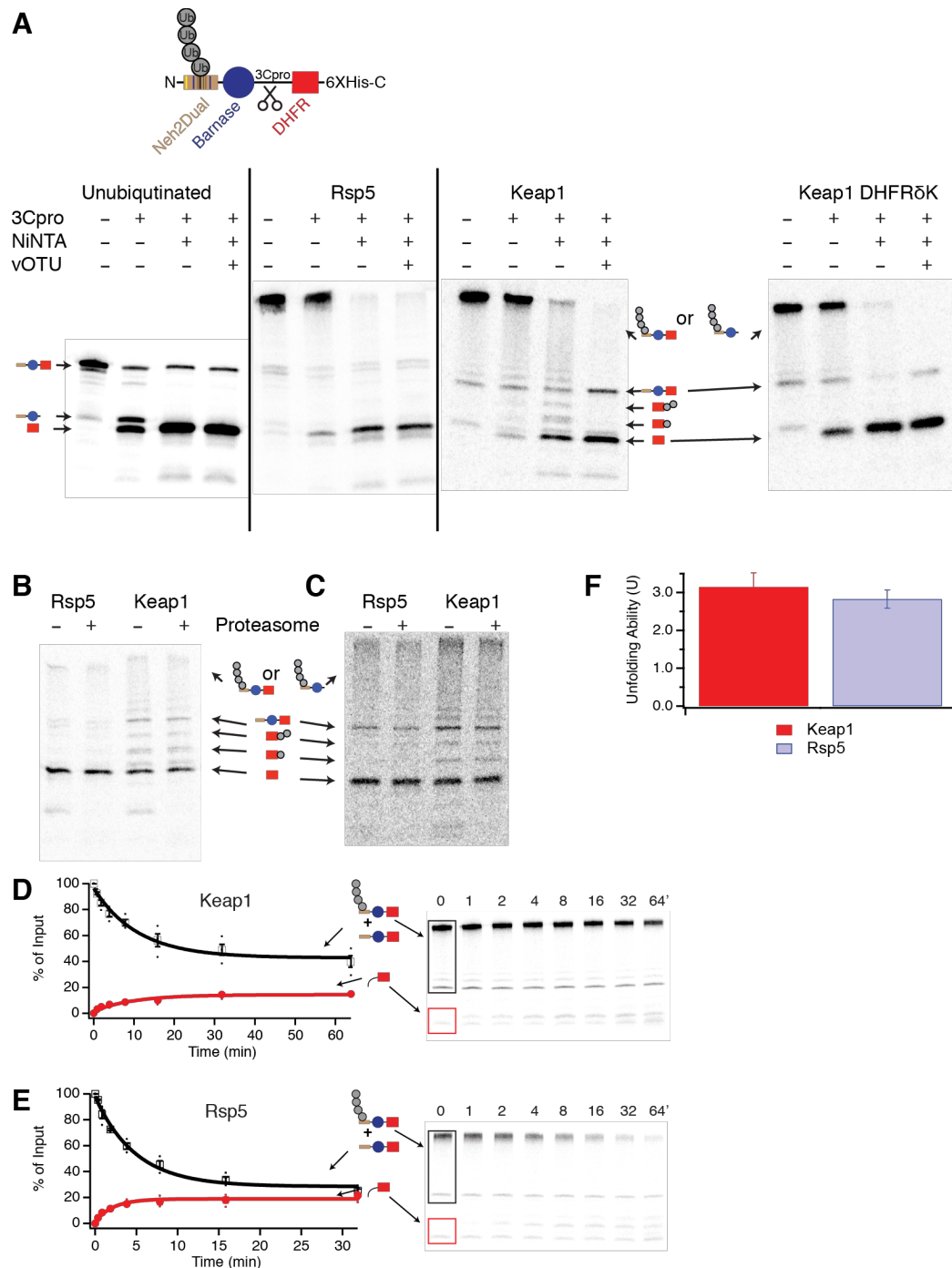
Figure 6. Substrate is polyubiquitinated on the degron, not the DHFR domain. A) Neh2Dual-BarnaseL89G-3Cpro-DHFR-His or Neh2Dual-BarnaseL89G-3Cpro-DHFR \delta K-His was ubiquitinated (or left unubiquitinated), cleaved with 3C-protease, and then repurified on NiNTA magnetic beads. After elution, the sample was either treated or mock-treated with vOTU to remove any ubiquitins on the DHFR domain. DHFR \delta K sample was ubiquitinated in the presence of 500 \mu M NADPH. Lines indicate separate gels. B) The purified DHFR fragment from A was incubated with 100 nM wild-type proteasome for 1 hr at 30 ^{\circ} C. There was no change in intensity of any of the DHFR bands, indicating that these DHFR fragments are not degraded or
