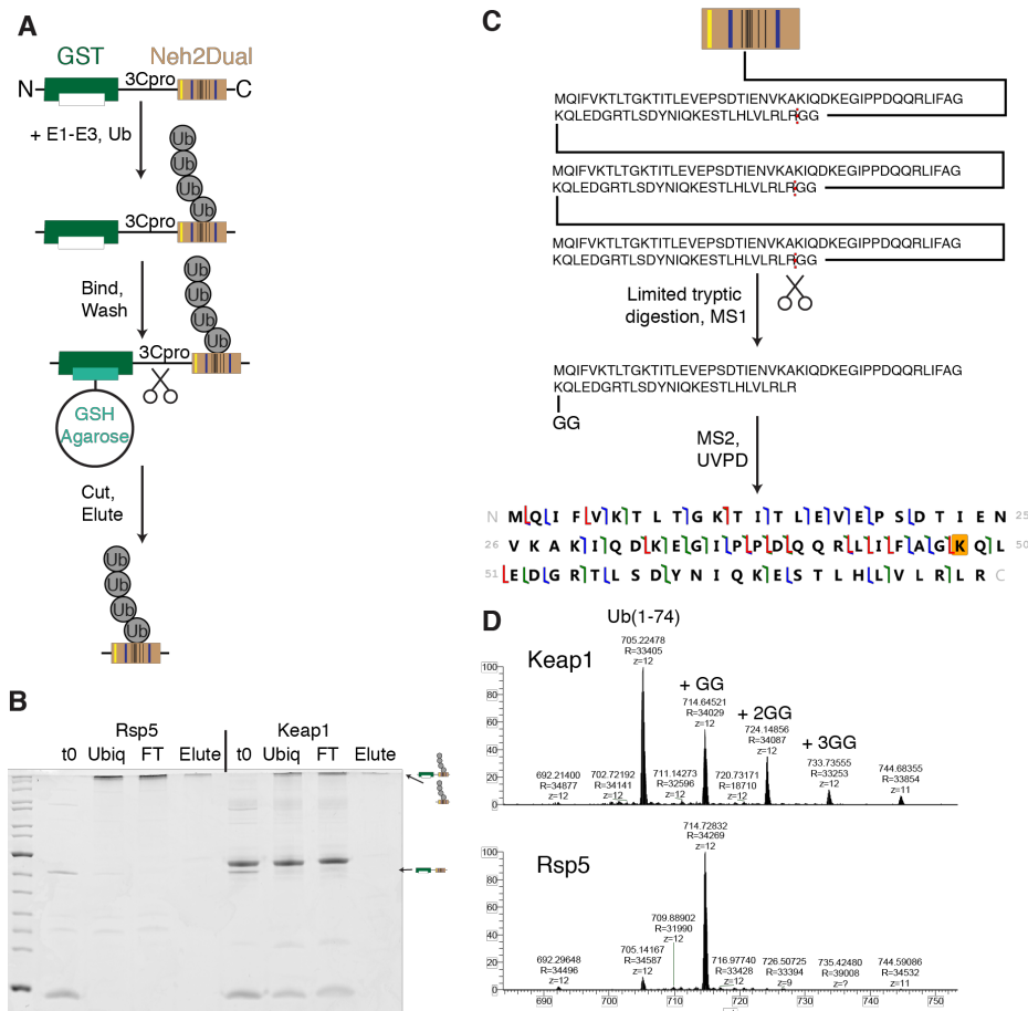
Figure 5. Characterization of Rsp5- and Keap1-ubiquitinated substrates. A) Schematic depiction of GST-Neh2Dual substrate preparation. Yellow bar indicates Rsp5 binding site, blue bars Keap1 binding sites and black bars lysines in the Neh2 domain. Substrate was ubiquitinated with either Rsp5 or Keap1, bound to GSH-agarose beads, washed to remove free ubiquitin chains and components of the ubiquitination reaction, and then eluted by cleavage with GST-tagged HRV 3C protease. B) Coomassie-stained gel showing ubiquitination (t0 is a sample taken immediately after the reaction was initiated by addition of ubiquitin) and purification of the GST-Neh2Dual sample. Final elutions contain almost exclusively polyubiquitinated Neh2Dual with no contaminating free ubiquitin. Strong band just above the full-length substrate in Keap1 lanes is ovalbumin, a component of the ubiquitination buffer. C) Schematic depiction of middle-down mass spectrometry approach. Substrate (shown here as Ub 3 attached to one lysine in Neh2Dual) was subjected to limited tryptic digestion to cleave ubiquitin prior to glycine 75 to generate ubiquitin(1-74) monomers. Here the proximal or middle ubiquitin is shown after digestion; this ubiquitin contains a diglycine appended to K48 that was derived from the distal ubiquitin in the chain. The distal ubiquitin would generate a ubiquitin(1-74) monomer lacking any diglycine modifications. Following cleavage, MS1 was used to identify the number of glycine modifications, and MS2 analysis with UVPD was used to determine the most likely site(s) of modification. D) Ub(1-74) monomers detected for Keap1 and Rsp5. For Keap1, monomers containing between zero and three diglycines were detected, indicating substantial branching, while for Rsp5, only monomers lacking or containing a single diglycine were detected, indicating linear chains.
