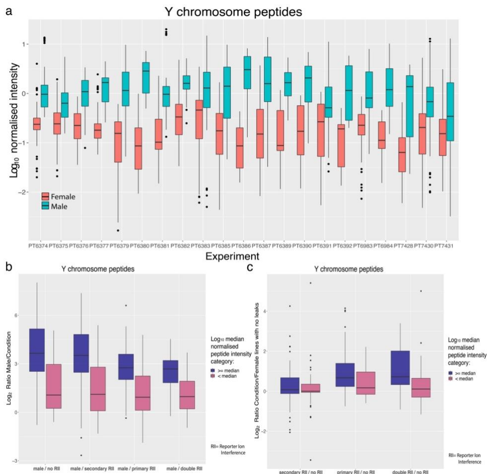
Figure 6 – TMT channel leakage analysis: (a) Box plot showing the median normalised intensity of Y chromosome specific peptides detected for both female and male cell lines across all 21 TMT batches. (b) Box plot of ratios for Y chromosome specific peptides, stratified by the median log 10 normalised intensity. (c) Box plot of ratios for Y chromosome specific peptides, stratified by the median log 10 normalised intensity, comparing leakage conditions vs channels without leaks.
