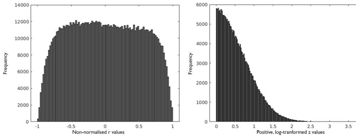
FIGURE S2. Distribution of values in MPC_{HIST} matrix. ( Left ) Frequency of r values calculated by Pearson product moment correlation coefficient of the nodal intensity profiles, controlling for the average intensity profile. ( Right ) Frequency of positive z values following log transformation of r values.
