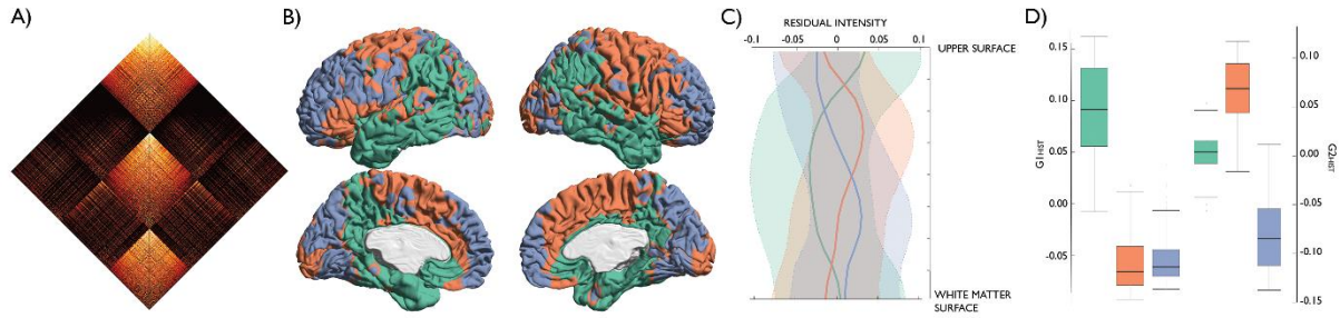
FIGURE S9. Community structure of the MPC HIST . (A) MPC HIST matrix sorted by community membership. (B) Modular decomposition of MPC HIST projected on the BigBrain midsurface. (C) Mean \pm sd of residual intensity profile for each module, after correction for the midsurface y-coordinate and demeaning. (D) Boxplot depicts the unique positions of modules along the first two principal gradients.
