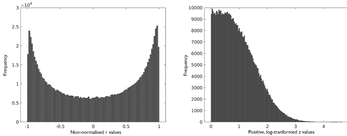
FIGURE S6. Distribution of values in MPC_{MRI} matrix. ( Left ) Frequency of r values calculated by Pearson product moment correlation coefficient of the nodal intensity profiles, controlling for the average intensity profile. ( Right ) Frequency of positive z values following log transformation of r values.
