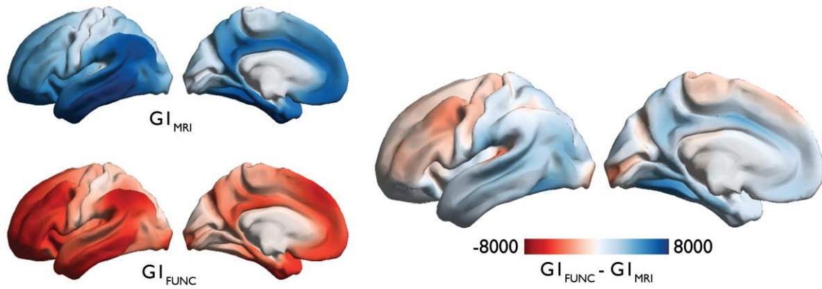
Figure S8: Differences in vertex ranks between G1_{MRI} ( blue ) and G1_{FUNC} ( red ).
