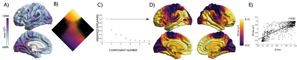
FIGURE S13. Independent replication of G1_{MRI} , using quantitative T1 relaxometry (qT1) images. (A) Mean qT1 intensity across subjects projected onto the cortical surface. (B) Gradient ordered normalised angle matrix. (C) Variance explained by embedding components. (D) First principal gradient ( G1_{MRI-QT1} ) projected onto conte69 midsurface. (E) Scatterplot depicting the strong correlation between the G1_{MRI} and G1_{MRI-QT1} ( r=0.81 , p<0.001 ).
