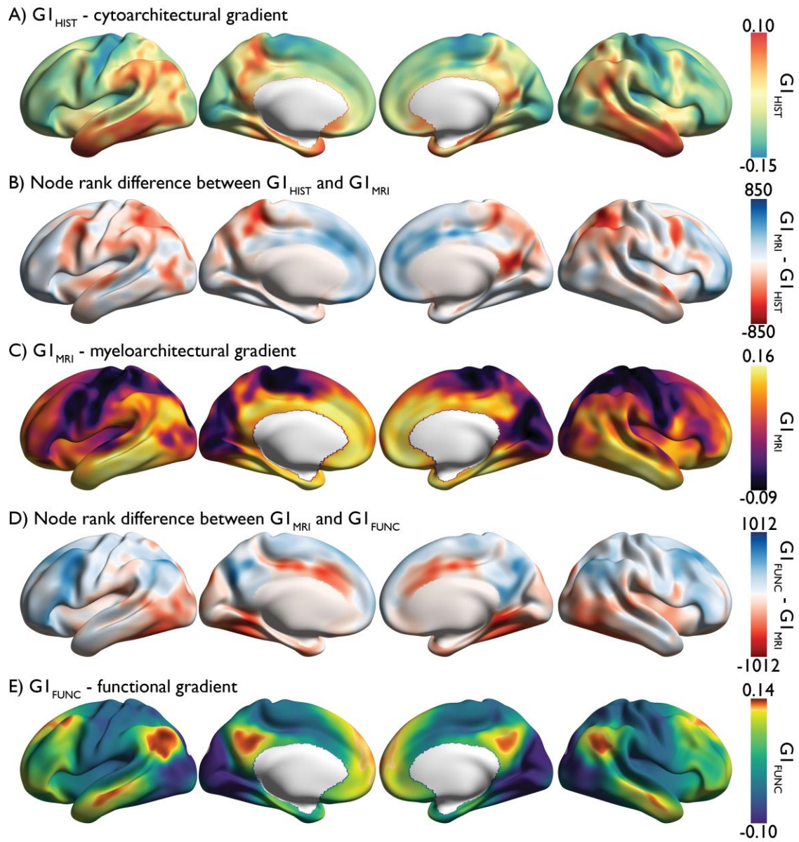
Figure S5: Principal gradients and node-rank differences projected on inflated cortical surfaces.
