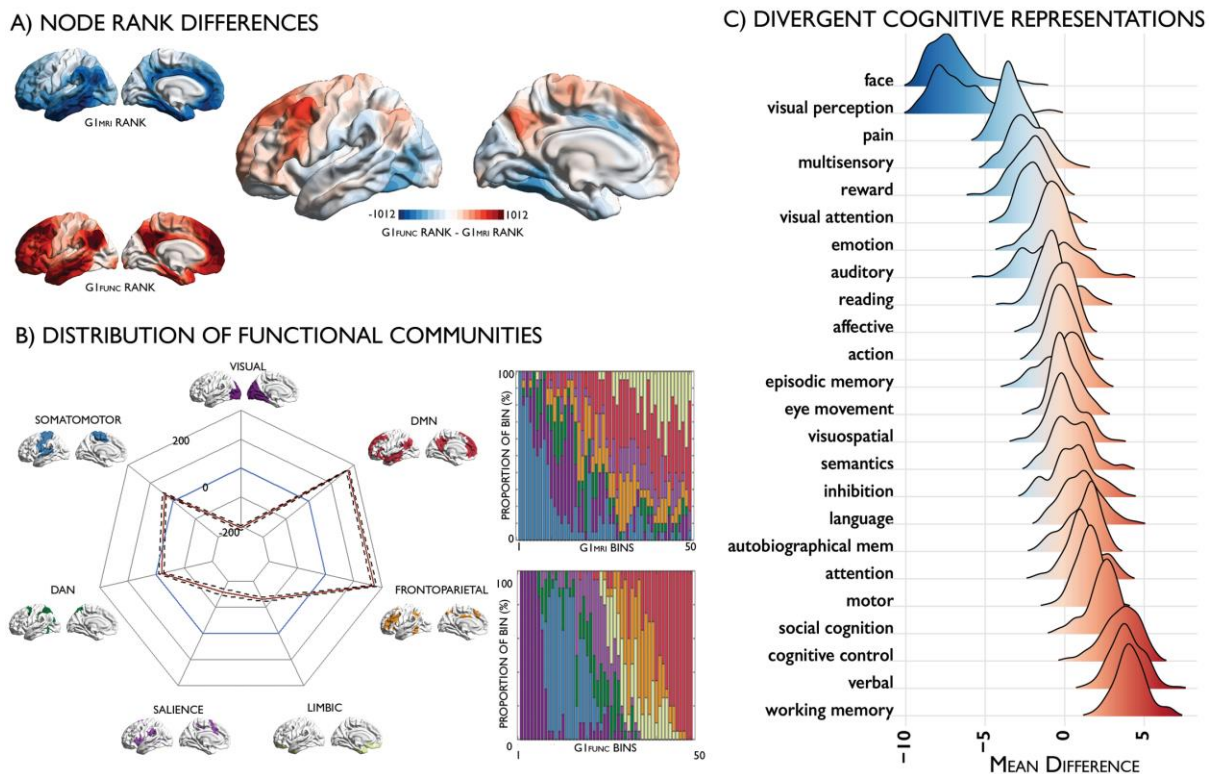
Fig 5. Divergent representations of the cortical hierarchy derived from microstructure and function. (A) Differences in nodal ranks between G1_{MRI} (blue) and G1_{FUNC} (red). (B) Radar plot depicting the difference in mean node ranks of functional communities [26] between G1_{MRI} (blue) and G1_{FUNC} (red), with 95% confidence intervals calculated across individuals presented with dotted lines; stacked bar plots depicting the proportion of each bin accounted for by intrinsic functional communities. (C) Meta-analysis maps for diverse cognitive terms were obtained from Neurosynth [28]. We calculated node-wise z-statistics, capturing node-term associations, and calculated the centre of gravity of each term along G1_{FUNC} and G1_{MRI} . The density plots depict the mean difference in the centre of gravity of meta-analysis maps in G1_{FUNC} and G1_{MRI} space across subjects. In-vivo imaging data is openly available as part of the Human Connectome Project S-900 release ( https://www.humanconnectome.org/study/hcp-young-adult/document/900-subjects-data-release ).
