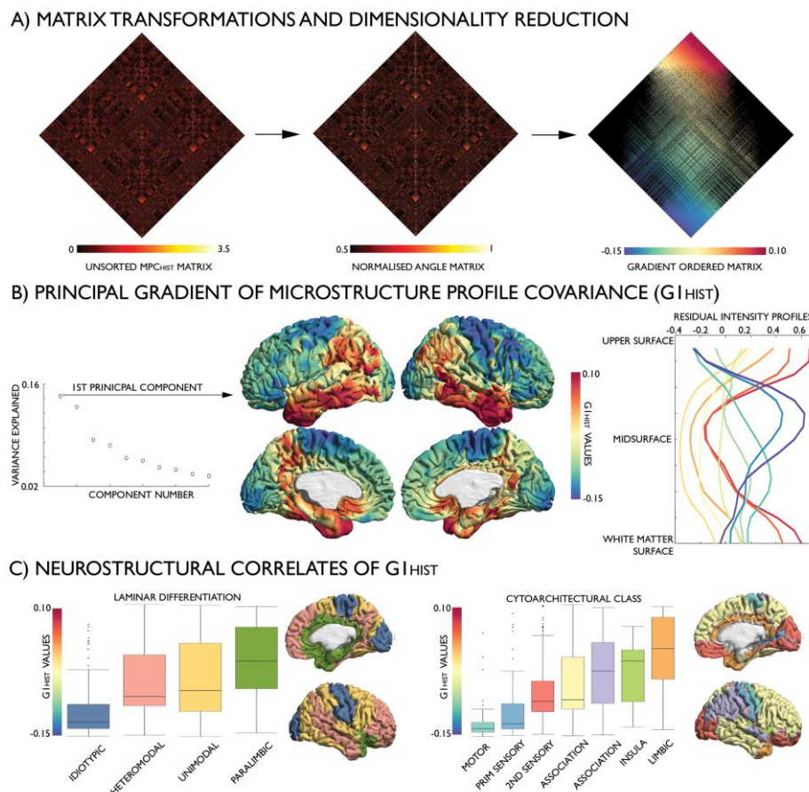
Fig 2. The principal gradient ( G1_{HIST} ) of the histology-based microstructure profile covariance matrix ( MPC_{HIST} ). (A) Identification: the MPC_{HIST} matrix was transformed into an affinity matrix, which captures similarities in microstructural profile covariance between nodes; this affinity matrix was subjected to diffusion map embedding, a non-linear compression algorithm that sorts nodes based on MPC_{HIST} similarity. (B) Variance explained by embedding components ( left ). The first component, G1_{HIST} , describes a gradual transition from primary sensory and motor ( blue ) to transmodal and limbic areas ( red ), corresponding to changes in intensity profiles, illustrated with the mean residual intensity profile across ten discrete bins of the gradient ( right ). (C) Spatial associations between G1_{HIST} and levels of laminar differentiation [ left ; [40]] and cytoarchitectural taxonomy [ right ; [13,41]], ordered by median. Histological data is openly available as part of the Big Brain initiative ( https://bigbrain.loris.ca/main.php ).
