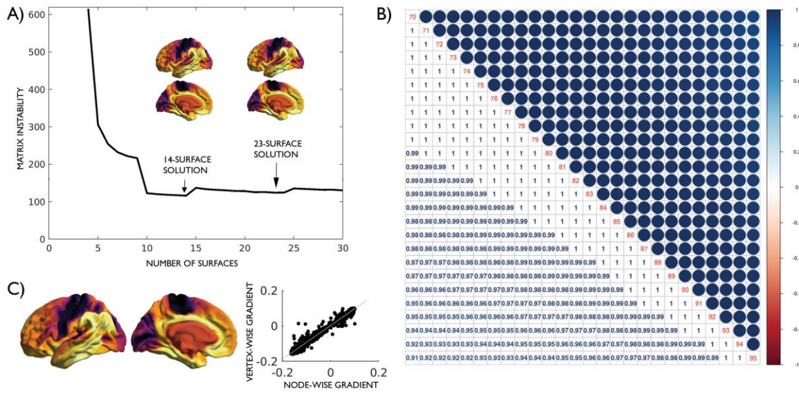
FIGURE S10. Robustness of G1_{MRI} to parameter variation. (A) MPC_{MRI} matrix instability using between 4 and 30 intracortical surfaces. G1_{MRI} was consistent regardless of the number of intracortical surfaces used, as shown by the strong spatial correlation of the 14- and 23-surface solutions ( r=0.98 , p<0.001 ). (B) Correlation matrix depicting the high correspondence of G1_{MRI} solutions with 70-95% row-wise matrix thresholding ( 0.91<r<1 , all p<0.001 ). (C) Estimation of G1_{MRI} from 20464 vertices resulted in a consistent G1_{MRI} to the 1012 parcel construction pipeline ( r=0.98 , p<0.001 ).
