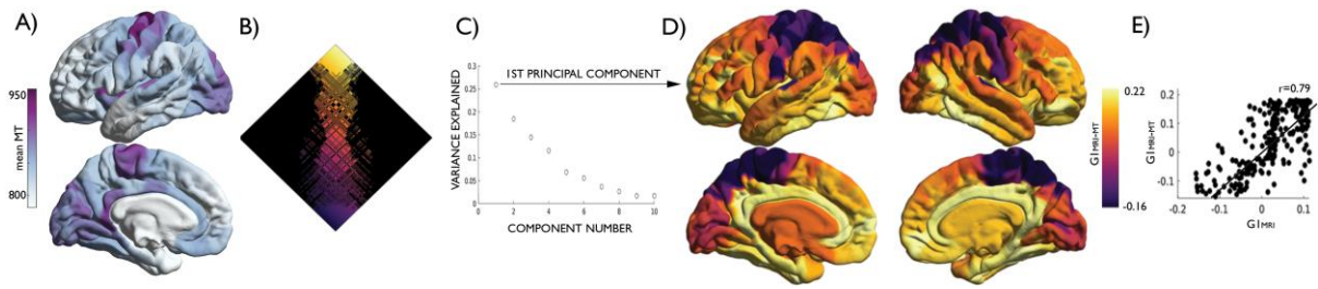
FIGURE S12. Independent replication of G1_{MRI} , using magnetisation transfer (MT) data. (A) Mean MT intensity across subjects projected onto the cortical surface. (B) Gradient ordered normalised angle matrix. (C) Variance explained by embedding components. (D) First principal gradient ( G1_{MRI-MT} ) projected onto conte69 midsurface. (E) Scatterplot depicting the strong correlation between the G1_{MRI} (reconstructed with the 308 parcellation scheme) and G1_{MRI-MT} ( r=0.79 , p<0.001 ).
