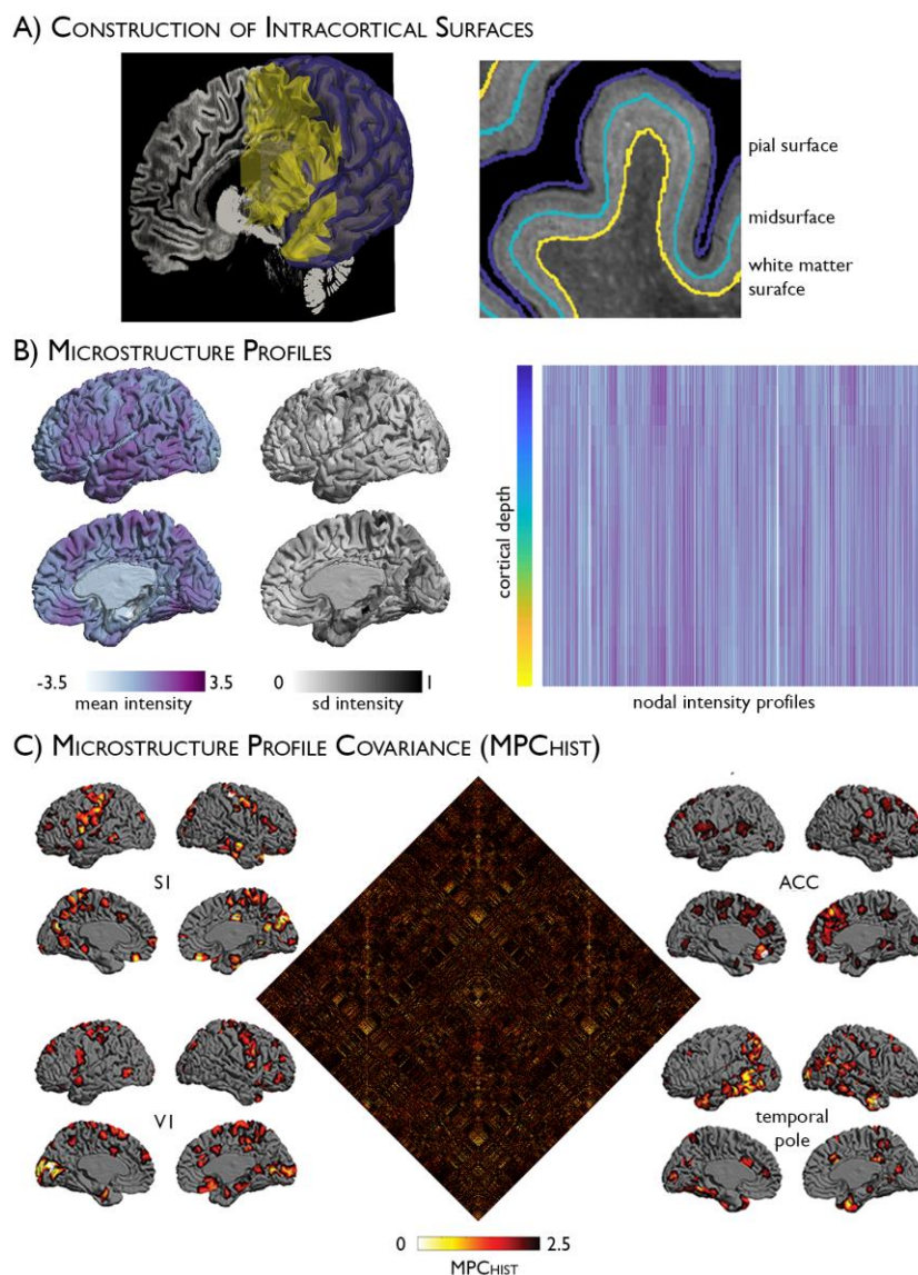
Fig 1. Histology-based microstructure profile covariance (MPC HIST ) analysis. (A) Pial (purple) and white matter (WM: yellow) surfaces displayed against a sagittal slice of the BigBrain (left) and with the midsurface (blue) in magnified view (right). (B) Mean and standard deviation (SD) in residual intensity at each node are displayed on the cortex (left). Cortex-wide intensity profiles were calculated by systematic intensity sampling across intracortical surfaces (rows) and nodes (columns). (C) The MPC HIST matrix depicts node-wise partial correlations in intensity profiles, controlling for the average intensity profile. Exemplary patterns of microstructural similarity from primary somatosensory (S1), anterior cingulate cortex (ACC), primary visual (V1) and the temporal pole. Seed nodes are shown in white. Histological data is openly available as part of the Big Brain initiative ( https://bigbrain.loris.ca/main.php ).
