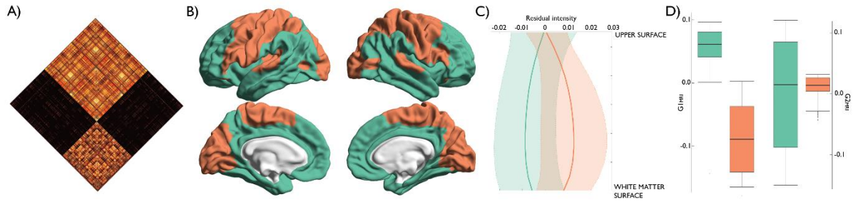
FIGURE S11. Community structure of the MPC MRI . (A) MPC MRI matrix sorted by community membership. (B) Modular decomposition of MPC MRI projected on the conte69 midsurface. (C) Mean \pm sd of residual intensity profile for each module, after demeaning. (D) Boxplot depicts the unique positions of modules on the first, but not the second, principal component.
