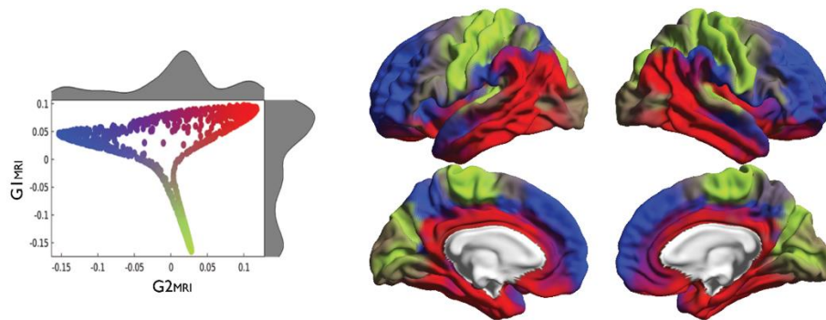
FIGURE S7. (A) The second principal component, accounting for 11.7% of variance in MPC MRI components, projected on the conte69 midsurface. (B) Scatterplot depicting the first two embedding gradients, with corresponding probability density functions. The second gradient divides the higher-order areas of the first gradient, insomuch that the cingulate, orbitofrontal cortex and the inferior temporal gyrus ( red ) are separated from the prefrontal cortex, precuneus, temporo-parietal junction and superior temporal gyrus ( blue ).
