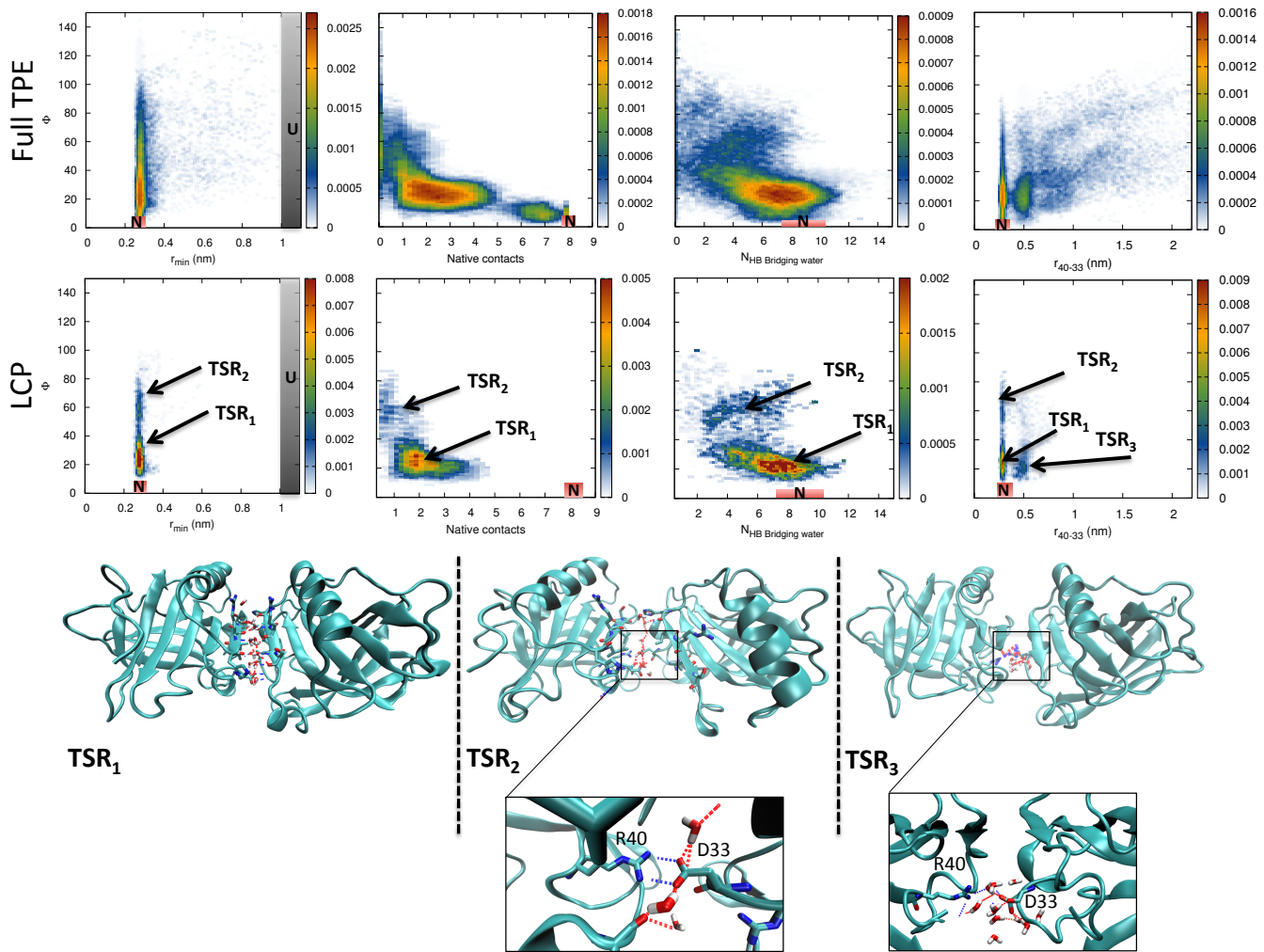
FIG. 4: Path density plots of \phi as a function of protein-protein minimum distance (col 1), native contacts (col2) number of hydrogen bond bridging waters (col3) and R40-D33 distance (col4) for the full transition path ensemble (full TPE) and least changed path ensemble (LCP) respectively. The third shows snapshots of configurations of the TSR_1 , TSR_2 and TSR_3 .
