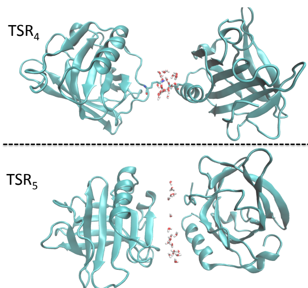
FIG. 9: Snapshots of configurations of the \text{TSR}_4 and \text{TSR}_5 .
