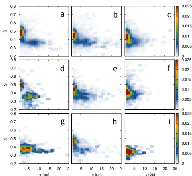
FIG. 10: Two dimensional histograms of the reorientation time \tau versus structural parameter S or water molecules residing at the native interface from NVE simulations performed in the a) native, b) transient near native (TSR 2 ) and c) unbound states at 300 K. Structural parameter-reorientation time correlation for the native state hydrophobic residues I147, L149 at d) native e) near native and f) unbound configurations. Structure reorientation correlation for the hydrophilic residue D33 at g) native, h) near native, and i) unbound configurations.
