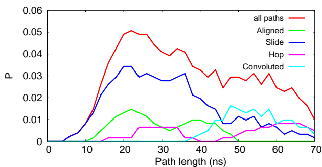
FIG. 1: Path length distribution of the N \rightleftharpoons U path ensemble and for the different observed mechanisms.
