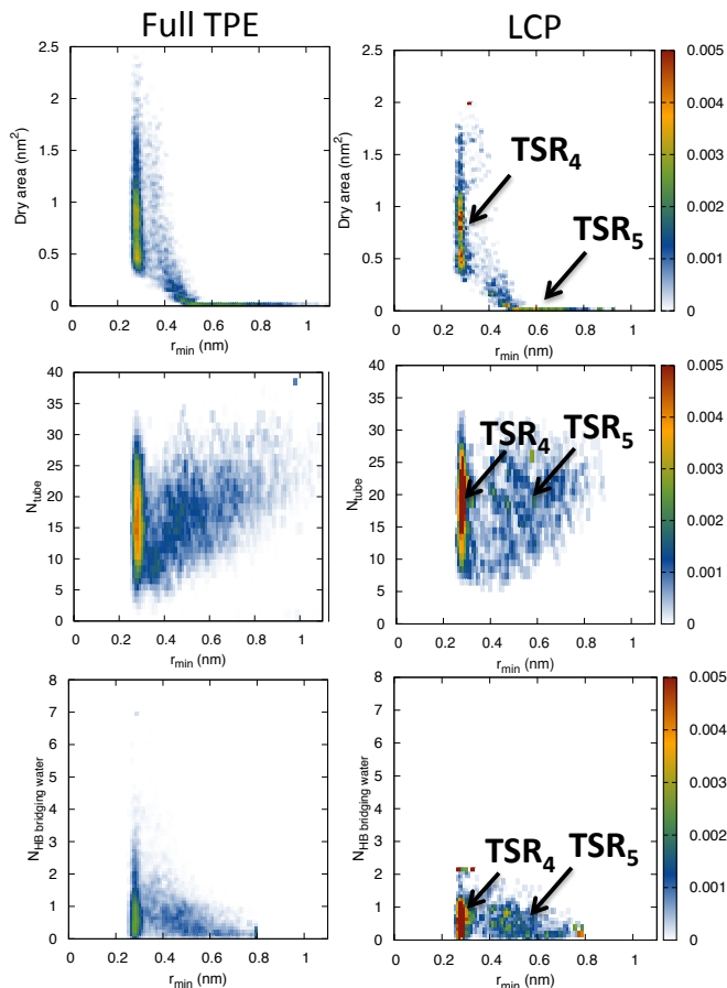
FIG. 8: Transition Path Ensemble and Least Changed Path density plots of the number of dry area vs protein-protein minimum distance (up), number of waters in the tube of radius 0.8 nm vs protein-protein minimum distance (middle) and the Number of hydrogen bond bridging waters vs protein-protein minimum distance (bottom) for the TPE (left) and the LCP (right).
