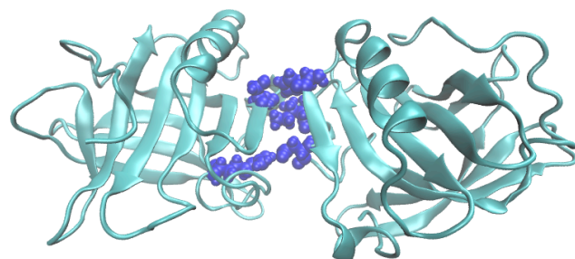
FIG. 3: Structure of an on pathway transiently formed intermediate. In blue are highlighted the long-lived contacts H146-S150, R40-D33, I29-S150.
