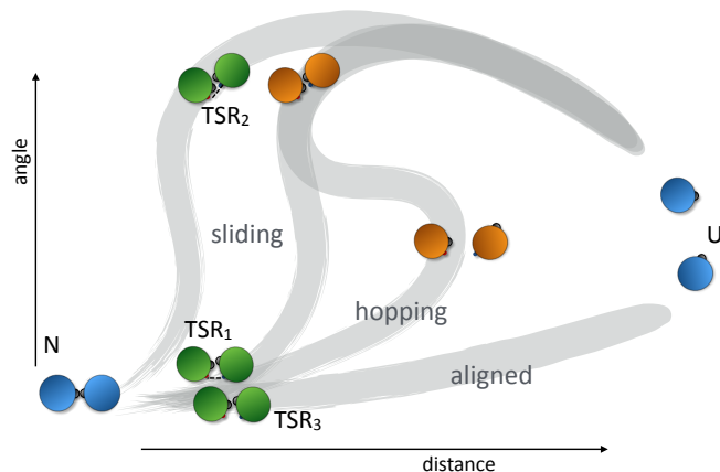
FIG. 2: Cartoon network of transitions and respective TSRs during the full dissociation/association process.
