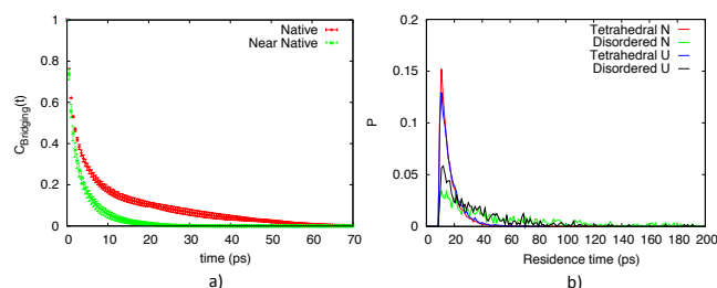
FIG. 11: a) Hydrogen bond bridge survival correlation function between any amino acid pair of the interface for native (red) and transient near native states (green) at 300 K. b) Distribution of residence times for the tetrahedral and disordered water population.
