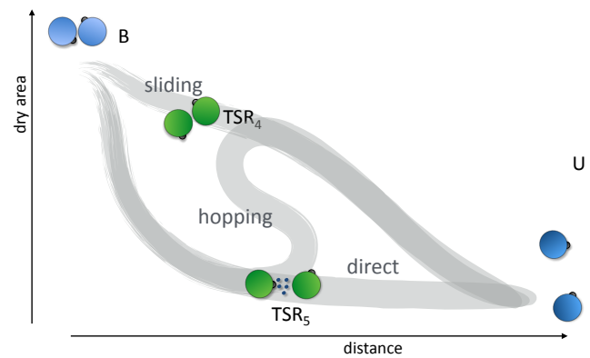
FIG. 7: Cartoon network of transitions and respective TSRs during the non specific dissociation/association process. We identify three types of mechanisms: a direct, hopping, and sliding mechanism.
