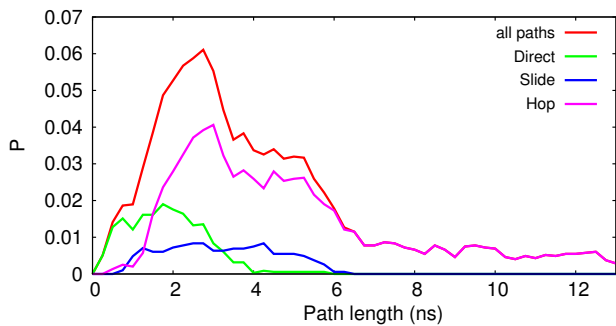
FIG. 6: Path length distribution of the B \rightleftharpoons U transition path ensemble with respect to the different underlying mechanisms. In red are all paths of the path ensemble, in green, blue, magenta, the ones corresponding to the direct, slide, hop dissociation/association.
