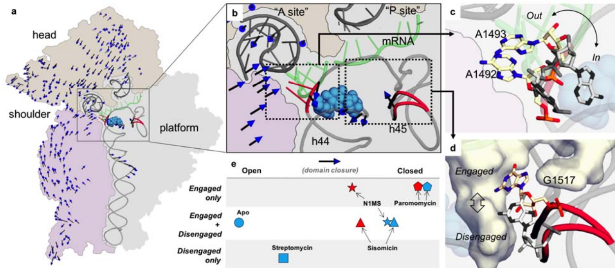
Figure 3. Sisomicin and N1MS binding to the 30S decoding complex induces an intermediate state of 30S domain closure. (A) The 30S ribosomal subunit illustrating the location of the drug binding pocket and the site of the h44-45 interactions. The drug is shown with blue spheres. The 30S subunit contour is shown with three different colored regions of interest, and the portion of the rRNA making helices h44 and h45, the ASL Phe and mRNA moieties are shown as gray ribbons. The first principal component (see Text ) is displayed as a vector field from the ensemble average structure. Note that smaller displacements were filtered out, and the arrows displayed are arbitrarily scaled, for clarity. More local motions of interest are further highlighted in red in the decoding center. (B) Detailed view of the decoding center displaying the drug binding pocket, where A1492 and A1493 (red sticks in left box) are displaced in response to aminoglycoside binding. The two h45 states, engaged and disengaged are also shown on the right (red ribbon in right box). (C) Detailed view of the flipping bases, in the context of the decoding center where the A-site tRNA (top left, gray), the mRNA (green) can be seen close to the outward flipped bases, and the aminoglycoside molecule (blue sphere) is seen superposed with the inward flipped state of the same bases. (D) Engaged and disengaged conformations of h45. The pocket in which G1517 is engaged, made in part by h44, is shown as a surface. Proximity to the drug (spheres in the background) binding site is apparent. (E) Ordering of the apo-30S (circle) structure and the streptomycin- (square), sisomicin- (triangle), N1MS- (star) and paromomycin- (pentagon) 30S decoding complex structures. Blue represents cryogenic structures, red represents ambient temperature structures studied along the 1st principal component extracted from their conformational ensemble. The vertical scale shows h45 disengagement, engagement or equilibrium in the corresponding crystal structure.
