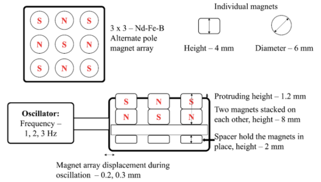
Fig. 1. Illustration of the alternate pole magnet array, made up of Nd-Fe-B permanent rare earth magnets, which was used for the induction of magneto mechanical cytotoxicity in cancer cells. Dimensions of the magnet used (height, diameter) and the populated magnet array (cross section) connected to the oscillator are provided.
