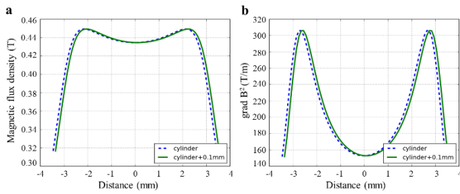
Fig. 5. Gradient flux density at culture well surface (adherent cell layer) during horizontal oscillation of the magnetic array. (a) 2D plot of the magnetic field (flux density) for 0 mm (x axis) and 0.1 mm shifted along the y-axis. (b) The field gradient (gradient flux density) for 0 mm (x axis) and 0.1 mm shifted along the y-axis.
