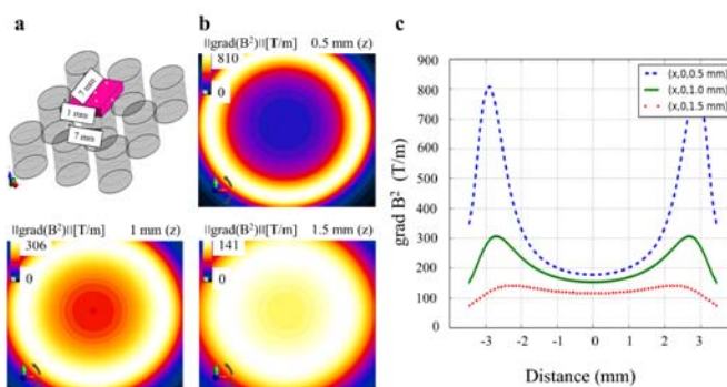
Fig. 4. Modelling of gradient flux density above a static magnet. (a) 3D model of the 3 x 3 magnet array used for gradient flux density calculations. (b) The field gradient distribution (gradient flux density) at 0.5, 1, and 1.5 mm along the z -axis (vertically above centre of magnet, x = y = 0 ). (c) 2D plot of the field gradient distribution (gradient flux density) across the midline of a magnet at 0.5, 1 and 1.5 mm above the magnet face.
