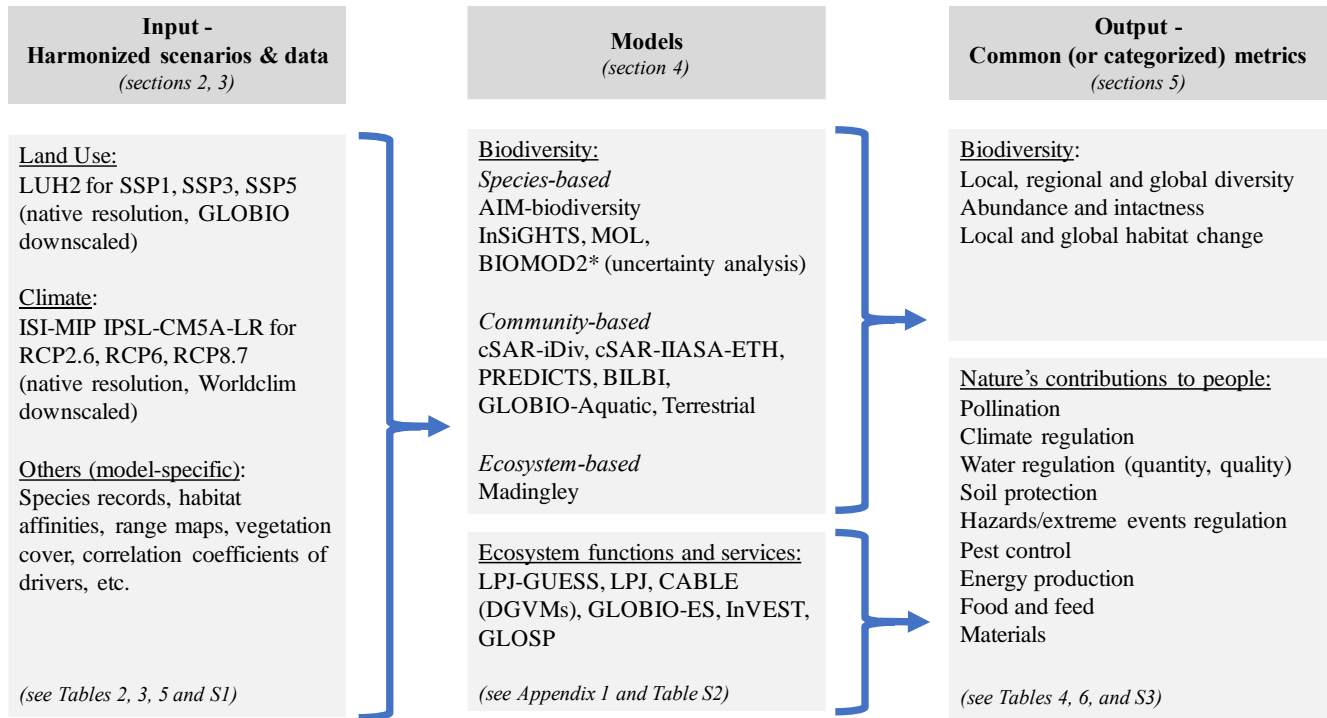
Figure 1: Input-models-output flowchart of BES-SIM.
