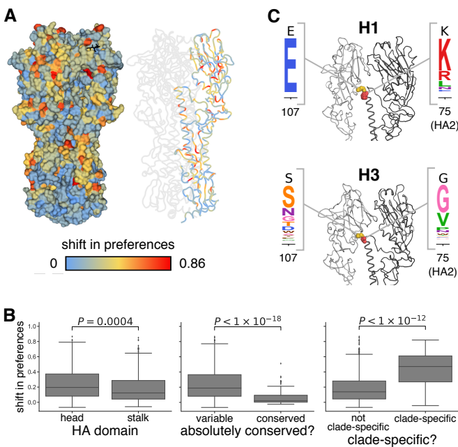
Fig. 8. Sites with strongly shifted amino-acid preferences between H3 and H1 HAs. (A) The shift in amino-acid preferences between the H3 and H1 HA at each site as calculated in Figure 7C is mapped onto the structure of the H3 HA. (B) Amino-acid preferences of sites in the stalk domain are less shifted than those in the head domain. Sites absolutely conserved in all 18 HA subtypes are less shifted than other sites. Sites with one amino-acid identity in the clade containing H1, H2, H5, and H6 and another identity in the clade containing H3, H4, and H14 are more shifted than other sites. (C) Sites 107 and 75(HA2) help determine the different orientation of the globular head domain in H1 versus H3 HAs. These sites are shown in spheres on the structure of H1 and H3 and colored as in panel (A), and the experimentally measured amino-acid preferences in the H1 and H3 HAs are shown. One monomer is in dark gray, while the HA1 domain of the neighboring monomer is in lighter gray.
