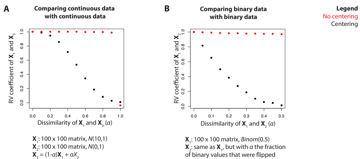
Fig. 4. Artificial data experiment in which the RV coefficient ( y -axis) is measured at different levels of similarity ( \alpha , x -axis), both with and without centering, for (A) two continuous datasets and (B) two binary datasets.
