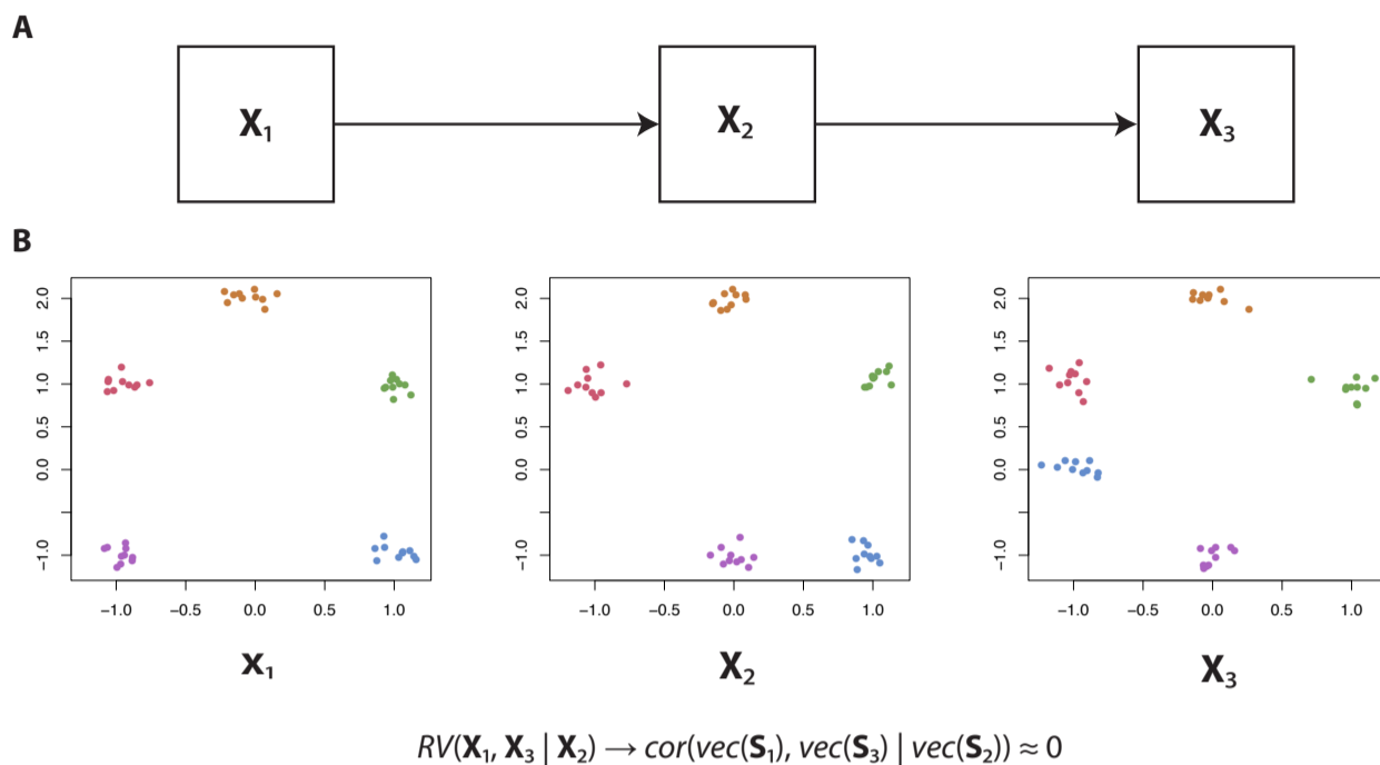
Fig. 3. Illustration of the partial matrix correlation. (A) We will create artificial data such that \mathbf{X}_1 influences \mathbf{X}_2 , which in turn influences \mathbf{X}_3 . (B) Artificial data consistent with the abovementioned causality, resulting in RV(\mathbf{X}_1, \mathbf{X}_3 | \mathbf{X}_2) \approx 0 .
