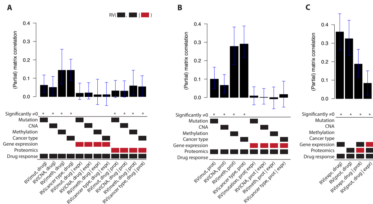
Fig. 6. The (partial) matrix correlations for different RV(\mathbf{X}_1, \mathbf{X}_2|\mathbf{X}_3) in the pharmacogenomics data. For each bar in the barplot, \mathbf{X}_1 and \mathbf{X}_2 are indicated by the black blocks, and \mathbf{X}_3 is indicated by the red block. A (partial) matrix correlation was significant when p < 0.01 . The error bars indicate the 99% confidence interval. Abbreviations: mut, mutation; meth, methylation; expr, gene expression; prot, proteomics; drug, drug response.
