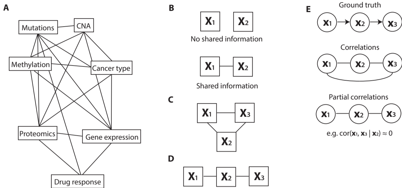
Fig. 1. High-level overview of this work. (A) The goal of this work is to infer a topology of relationships between pharmacogenomics datasets (an example topology is illustrated here). (B) When two datasets share information (i.e. when their RV coefficient is non-zero), we will indicate them as connected in a topology. (C) A topology of three datasets that all share information. We will convert this topology to the one depicted in (D) if the shared information between X_1 and X_3 is fully contained in X_2 . (E) To create these topologies we will draw on methods for inferring a topology between single variables using partial correlations. Top: the original causality graph. Middle: the topology as inferred using correlations. Bottom: the inferred topology using partial correlations.
