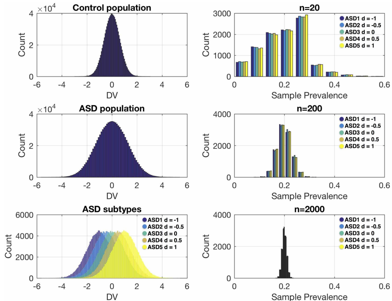
Figure 4: Simulation showing sampling variability and bias of enrichment of specific strata in small sample size studies. In this simulation we generated a control population ( n=1,000,000 ) with a mean of 0 and a standard deviation of 1 on a hypothetical dependent variable (DV). We then generated an autism population ( n=1,000,000 ) with 5 different autism subtypes each with a prevalence of 20% (e.g., n=200,000 for each subtype). These subtypes vary from the control population in effect size in units of 0.5 standard deviations, ranging from -1 to 1. This was done to simulate heterogeneity in the autism population that is reflective of very different types of effects. For example, the autism subtype 5 shows a pronounced increased response on the DV, whereas autism subtype 1 shows a pronounced decreased response on the DV. Across 10,000 simulated experiments, we then randomly sampled from the autism population sample sizes of n=20 , n=200 , and n=2000 , and computed the sample prevalence of each autism subtype. The ideal result without any bias would be sample prevalences of around 20% for each subtype. This 20% sample prevalence is approached at n=2000 , and to some extent at n=200 . However, small sample sizes such as n=20 shows large variability in sample prevalences of the subtypes and this can markedly bias the results of a case-control comparison. The code for implementing and reproducing these simulations is available at https://github.com/mvlombardo/effectsizesim .
