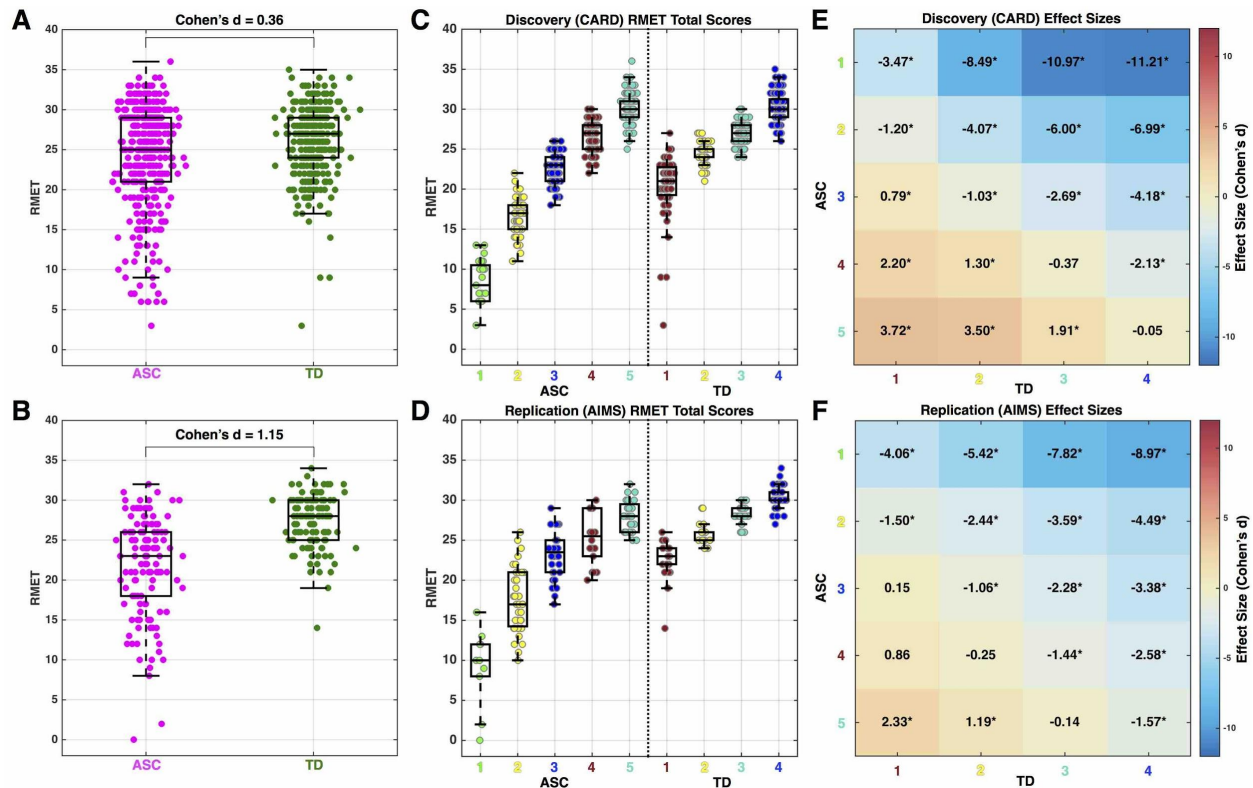
Fig 2: Case-control vs stratified model example with adult autism and mentalizing ability. This figure reports data from Lombardo et al. , (2016) 24 on two independent datasets of adults with autism and performance on an advanced mentalizing test, the Reading the Mind in the Eyes Test (RMET). Panels A (Discovery) and B (Replication) show case-control differentiation and the standardized effect size for each dataset. Panels C-F shows RMET scores and standardized effect sizes from the same two datasets after unsupervised data-driven stratification into 5 distinct autism subgroups and 4 distinct TD subgroups. autism subgroups 1-2 are highly impaired on the RMET, while autism subgroups 3-5 are completely overlapping in RMET scores with the TD population.
