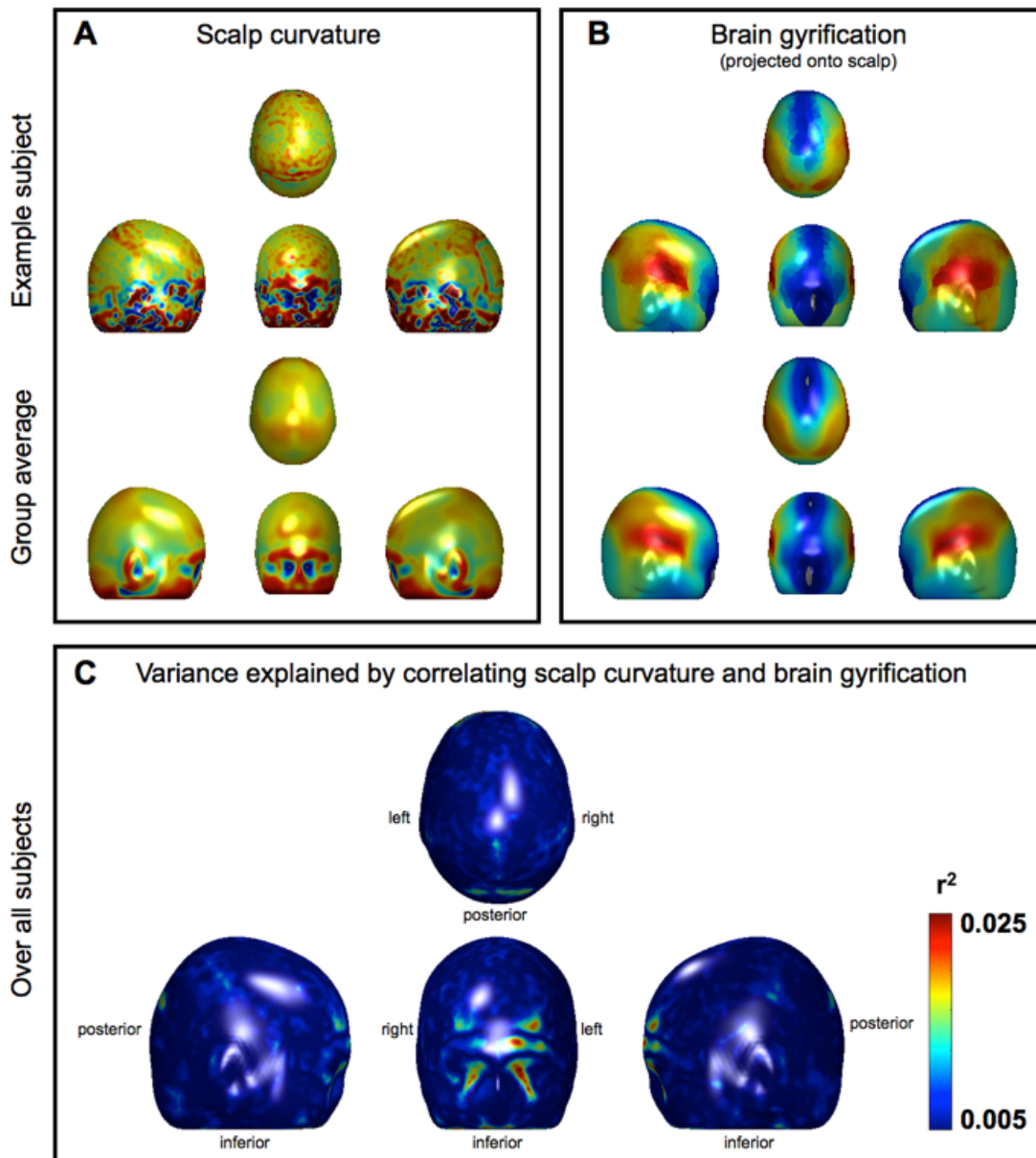
Figure 4: Scalp curvature, brain gyrification, and the variance explained by correlating the two. Panel A: Example scalp curvature data from a single subject (upper panel) and averaged over the entire cohort (lower panel). Red/Blue represents positive/negative (i.e. convex/concave) curvature values. Panel B: Example brain gyrification projected onto the scalp for a single subject (upper panel) and averaged over the entire cohort (lower panel). Red/Blue represents degree of gyrification (note large index values, in red, laterally over the Sylvian fissures). Panel C: Variance explained by correlating scalp curvature and brain gyrification. Note that the r^2 values are very small; the “strongest” effects only explain about 0.025% of the variance (leaving 97.5% unexplained). The largest “effects” are also marginalised to the facial region, which is irrelevant to a great number of phenological accounts and probably an artefact. All data have been projected onto the mean head surface.
