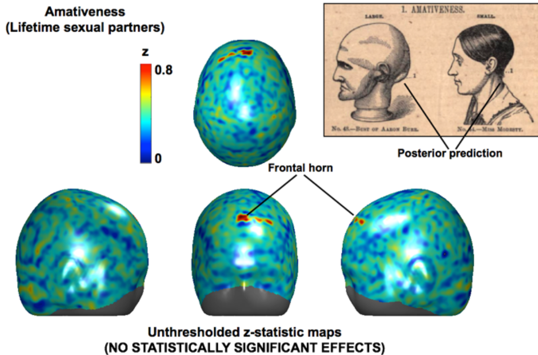
Figure 5: Illustration of over-interpreting null results. The scalp projections show an unthresholded z-statistic map of correlations between local scalp curvature and lifetime number of sexual partners, which has been overenthusiastically annotated with interpreted effects (i.e. the “frontal horn”). The results might be compared with those of the infamous “dead salmon” study, which highlighted the importance of correcting for multiple comparisons 34 . Please note that when thresholds for multiple comparisons were applied, none of the z-scores in this figure reached statistical significance. Also damning is the fact that the “frontal horn” area does not correspond to regions of interest predicted by 19 th century phrenologists. The upper-right panel depicts a prediction for “Amativeness” on the opposite side of the skull 25 .
