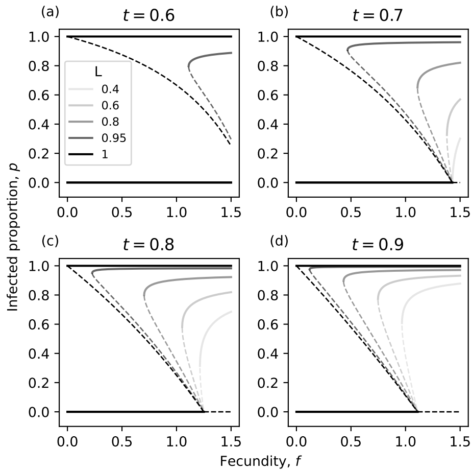
Figure 3. Equilibria of the diplodiploid model (Eq. (1)) as function of f , for different values of t (panel titles) and L (colours of the lines, see legend). Solid lines: stable equilibria. Dashed lines: unstable equilibria.
