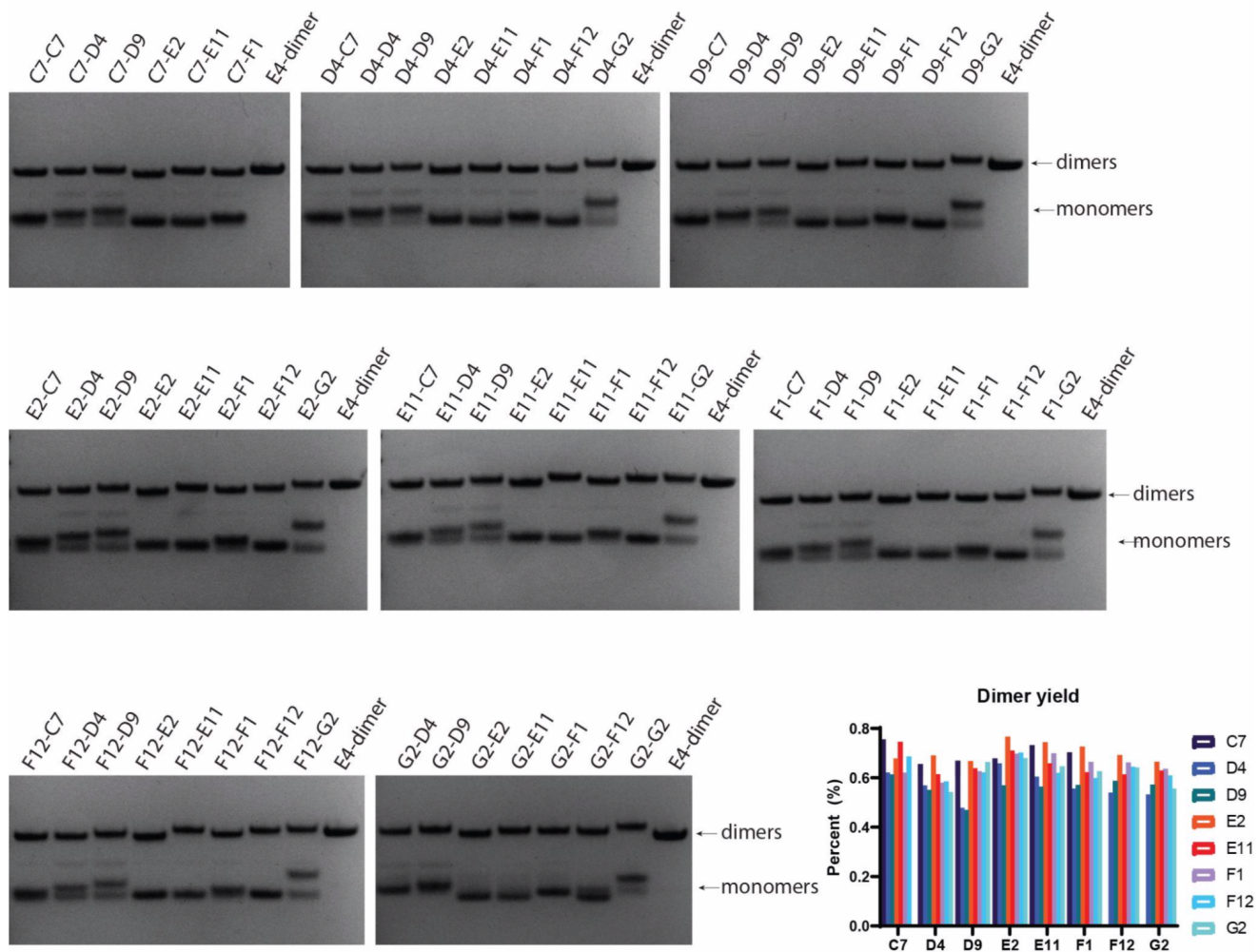
Fig. S14. SDS-PAGE analysis and Coomassie staining of nanobody dimers generated to rapidly screen for potentially neutralizing dimer pairs.
