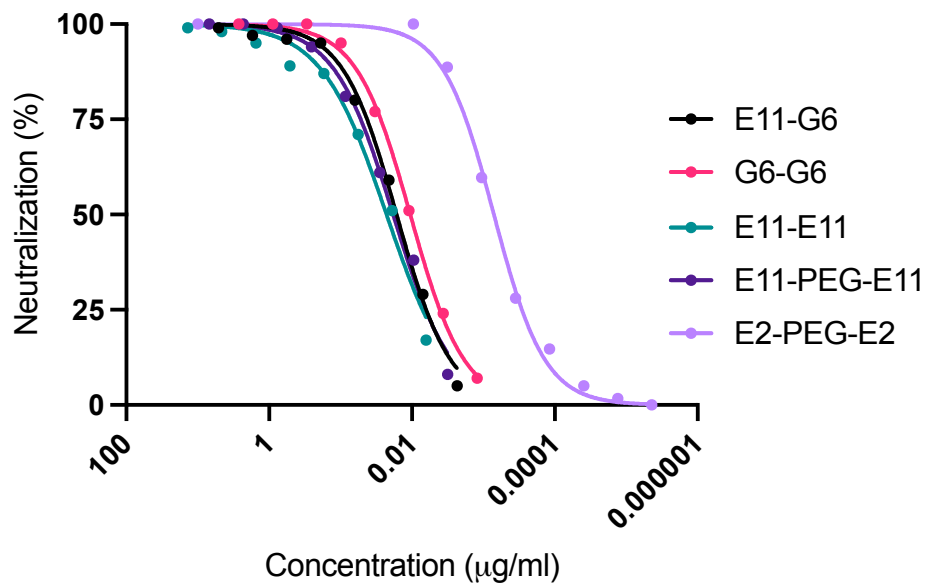
Fig. S12. Ultrapotent neutralization of SARS-CoV-2 by nanobody homo- and heterodimers. Neutralization of SARS-CoV-2 spike pseudotyped lentiviruses are shown for nanobody dimers generated by Cu-free strain-promoted azide-alkyne click chemistry (SPAAC) reaction. E11 and G6 homo- and heterodimers neutralized with similarly high potency. An E2 dimer (with a short PEG11 spacer, E2-PEG-E2) was ultrapotent, with an IC 50 of approximately 0.7 ng/ml (23 pM).
