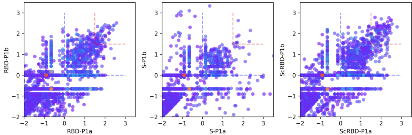
Fig. S11. Within-panning consistency estimation. We compare two “versions” of each nanobody variant that differ by degenerate bases introduced with the cloning primer when establishing the baseline library. RBD and ScRBD panning shows consistency in enrichment, but spike panning is less consistent.
