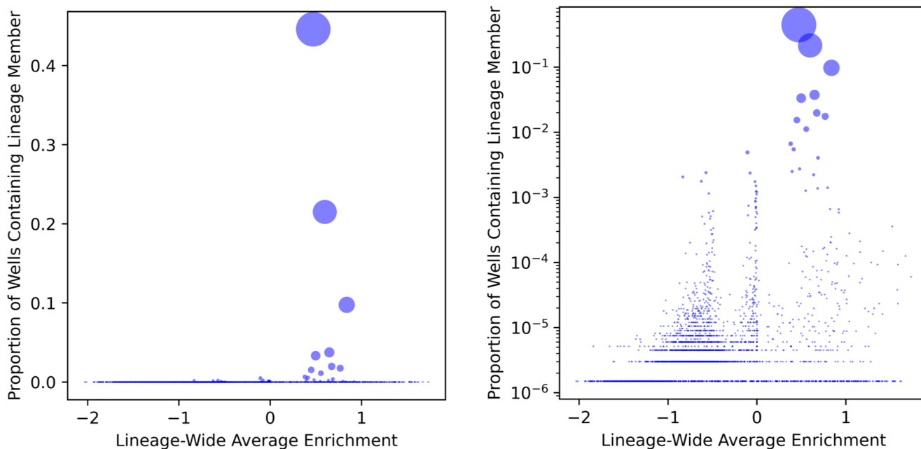
Fig. S15. Lineage enrichment vs sampling probability. Each bubble represents a lineage, showing the mean enrichment for each lineage vs the probability that a single well would contain a member from that lineage, after a second round of RBD panning, estimated from NGS frequency data (left: linear scale; right: log scale). The skewed size distribution of lineages, where a small number of lineages are extremely high frequency, shows that colony-based sampling approaches will not reach the lower frequency lineages. As an example, we would have had to screen nearly 500 colonies to have a >50% chance of discovering a member from the lineage of our highest affinity RBD binding nanobody (F1).
