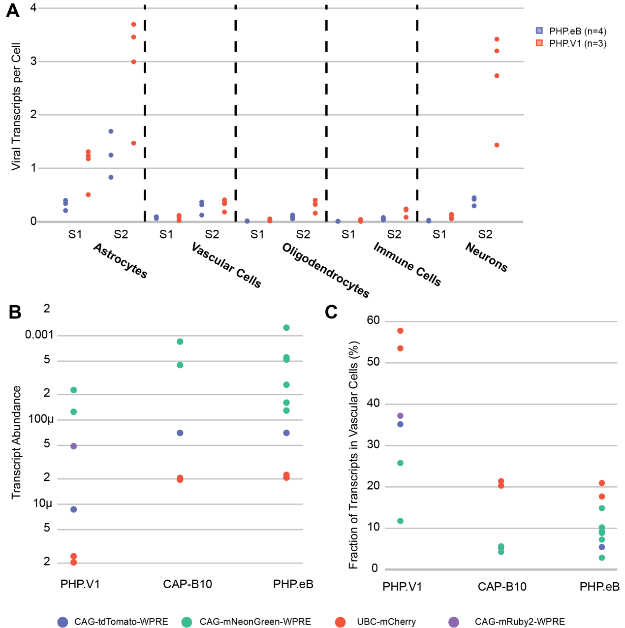
1165 Supplemental Figure 5. Transcript expression. (A) Viral transcript expression of different barcodes across two samples (S1, S2). Each point is a distinct barcode. (B) Viral transcript abundance in entire samples (viral transcripts / total transcripts) across different variants carrying different cargo. (C) Fraction of transcripts detected in vascular cells vs all other cell types.
