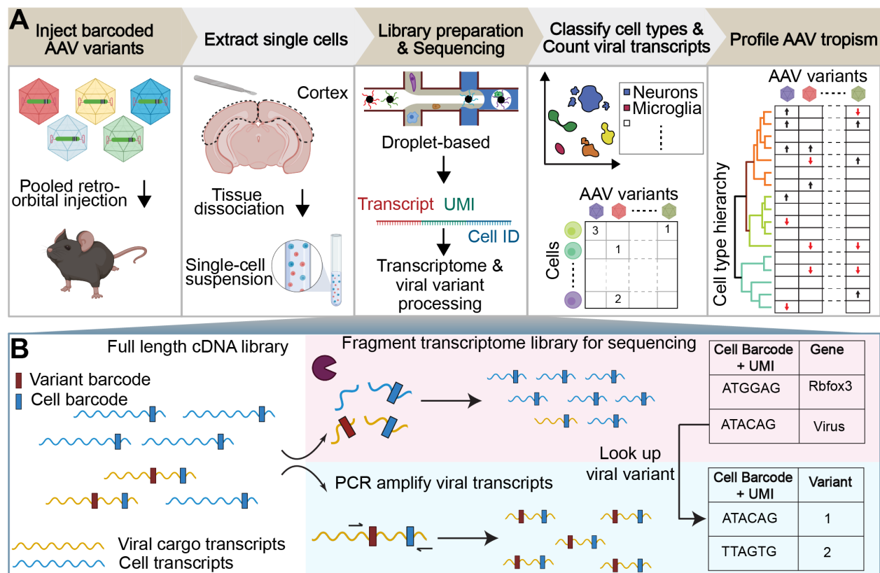
235 Figure 1. Workflow of AAV tropism characterization by scRNA-seq. (A) (I) Injection of a single AAV variant or multiple barcoded AAV variants into the retro-orbital sinus. (II) After 3–4 weeks post-injection, the brain region of interest is extracted and the tissue is dissociated into a single-cell suspension. (III) The droplet-based 10x Genomics Chromium system is used to isolate cells and build transcriptomic libraries (see B). (IV) Cells are assigned a cell-type annotation and a viral transcript count. (V) AAV tropism profiling across numerous cell types. (B) The full length cDNA library is fragmented for sequencing as part of the single-cell sequencing protocol (top). To enable viral tropism characterization of multiple rAAVs in parallel, an aliquot of the intact cDNA library undergoes further PCR amplification of viral transcripts (bottom). During cDNA amplification, Illumina sequencing primer targets are added to the viral transcripts such that the sequence in between the Illumina primer targets contains the AAV capsid barcode sequence. Viral cargo in the cell transcriptome is converted to variant barcodes by matching the corresponding cell barcode + UMI in the amplified viral transcript library (right). 240 245
