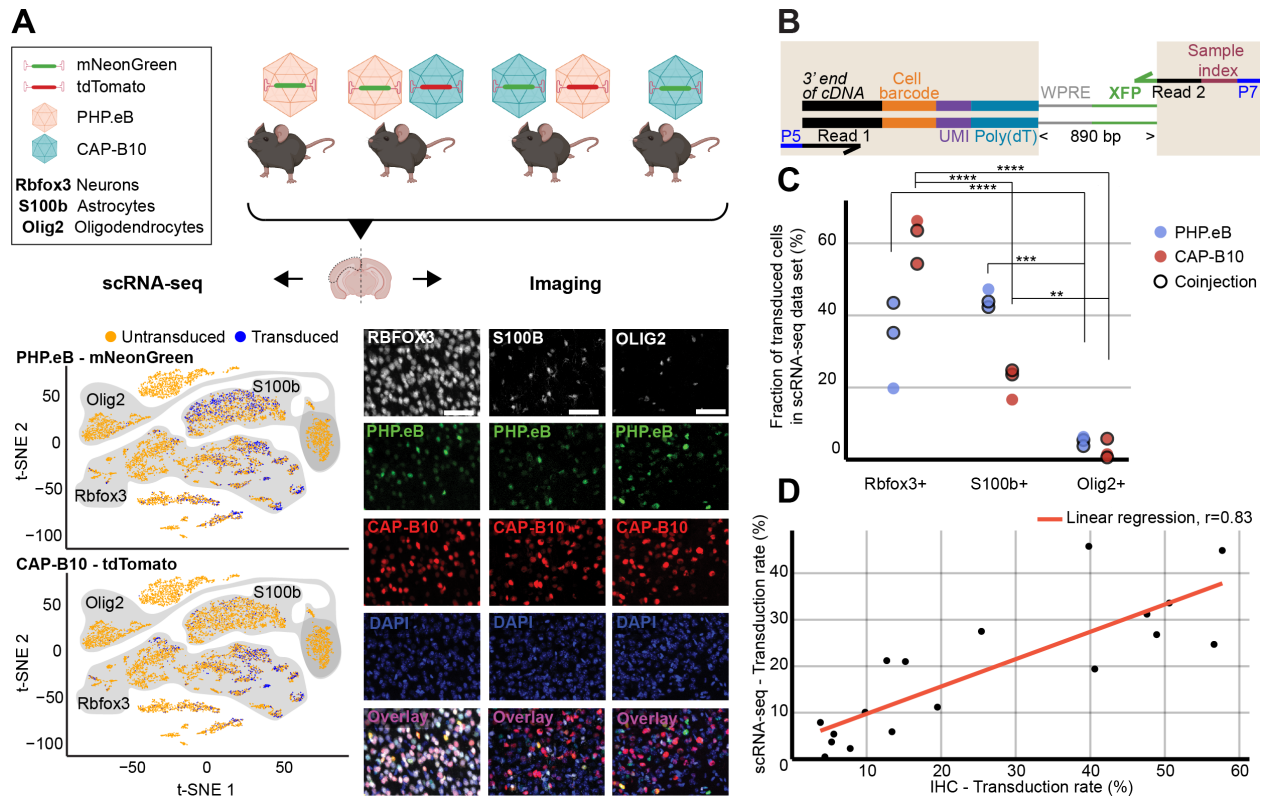
280 Figure 2. Comparison of viral tropism profiling with traditional IHC and scRNA-seq. (A) Overview of the experiment. Four animals were injected with 1.5 \times 10^{11} viral genomes (vg) packaged in AAV-PHP.eB and/or AAV-CAP-B10. The bottom panels show a representative dataset collected from an animal that was co-injected with AAV-PHP.eB and AAV-CAP-B10. The left side displays the scRNA-seq data set in the lower dimensional t-SNE space, with cells colored according to transduction status. The shaded areas indicate clusters with high expression of the corresponding gene marker. The right side shows representative confocal images of cortical tissue labeled with IHC. Scale bar, 50 \mu m. (B) Viral transcript recovery strategy. The shaded areas highlight sequences added during library construction. (C) The fraction of the total number of transduced cells labeled as expressing the corresponding marker gene. For each AAV variant, the results of a two-way ANOVA with correction for multiple comparisons using Sidak's test are reported with adjusted P-values (**** P \leq 0.0001 , *** P \leq 0.001 , and ** P \leq 0.01 are shown; P > 0.05 is not shown). (D) Comparison of transduction rates based on quantification via scRNA-seq or IHC. Transduction rate was calculated as (number of transduced cells in the group)/(total number of cells in the group). Each dot represents the transduction rate of neurons/Rbfox3+, astrocytes/S100b+, or oligodendrocytes/Olig2+ by AAV-PHP.eB or AAV-CAP-B10 in one animal. Histology data are averages across three brain slices per gene marker and animal. r indicates the Pearson correlation coefficient. 285 290 295
