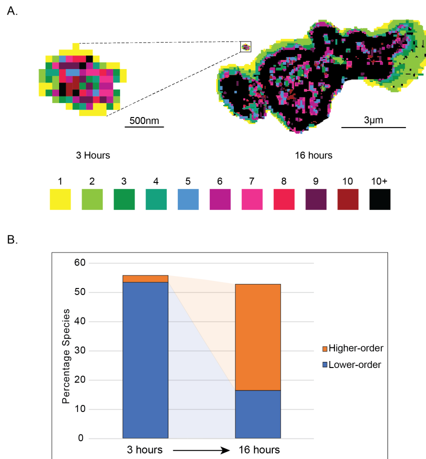
Figure 5. Distribution of oligomeric species in ARF19 condensates over space and time. (A) N&B analysis showing the spatial distribution of various oligomeric species in early (left) and late (right) ARF19 condensates. Each oligomeric species corresponds to a different color. The size of the early condensate relative to the late condensate can be seen in the box towards the top left of the late condensate. (B) N&B analysis showing the average percentage of higher-order and lower-order oligomers in ARF19 condensates in early condensates (left) and late condensates (right).
