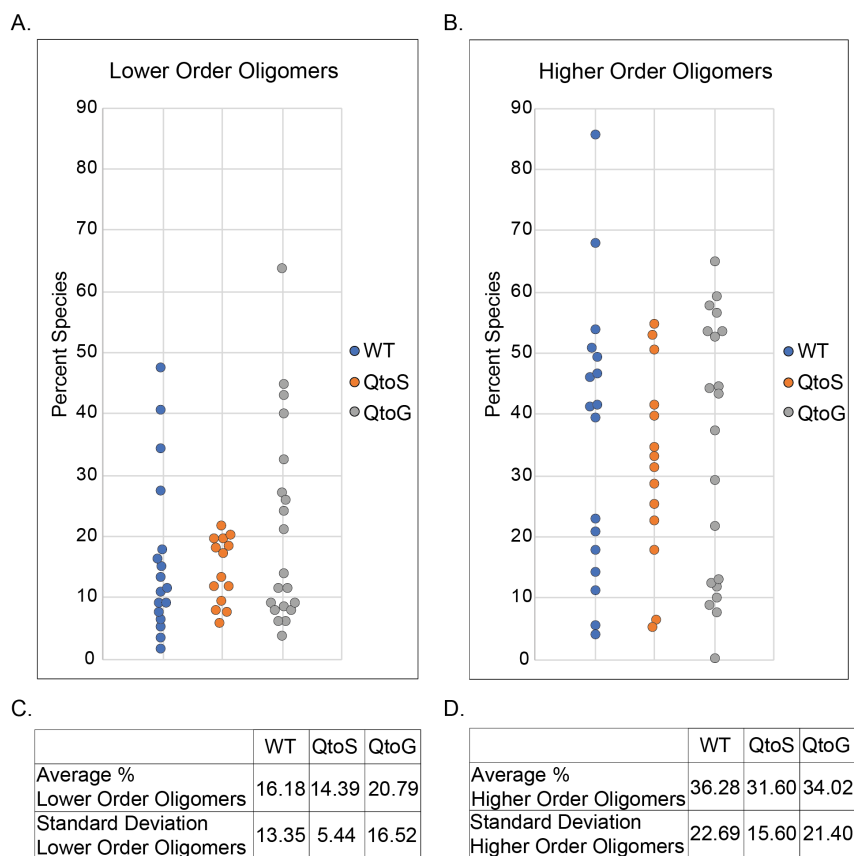
Figure 3. IDR composition has little impact on the oligomeric state of ARF19 condensates. (A) Each point represents the percent of monomers and dimers out of the total number of measured oligomers for an individual condensate. (B) Each point represents the percent of 10+-mers out of the total number of measured oligomers for an individual condensate. (C) A table summarizing the data from figure panel A. (D) A table summarizing the data from figure panel B. Statistical testing is not shown because none of the comparisons were statistically significant.
