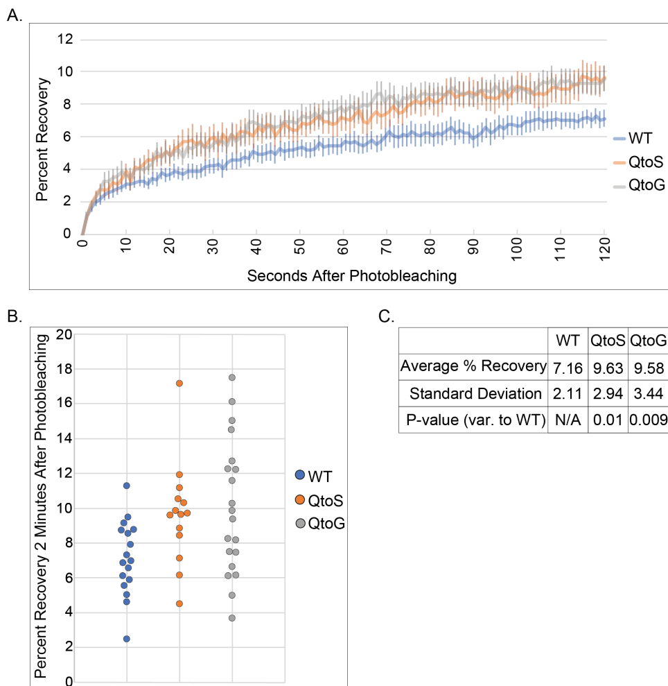
Figure 2. IDR composition impacts the fluidity of ARF19 condensates. (A) Average fluorescence recovery curves for the three ARF19 variants. Error bars report standard error of the mean. (B) Each point represents the percent recovery 2 minutes post-photobleaching of an individual condensate. For all FRAP experiments, only one half of the condensate was photobleached. N=17 (WT), N=14 (QtoS), N=20 (QtoG). (C) A table summarizing data from panel A. P-values were calculated using a two-sided t-test comparing the values from wild-type to each of the two IDR variants.
