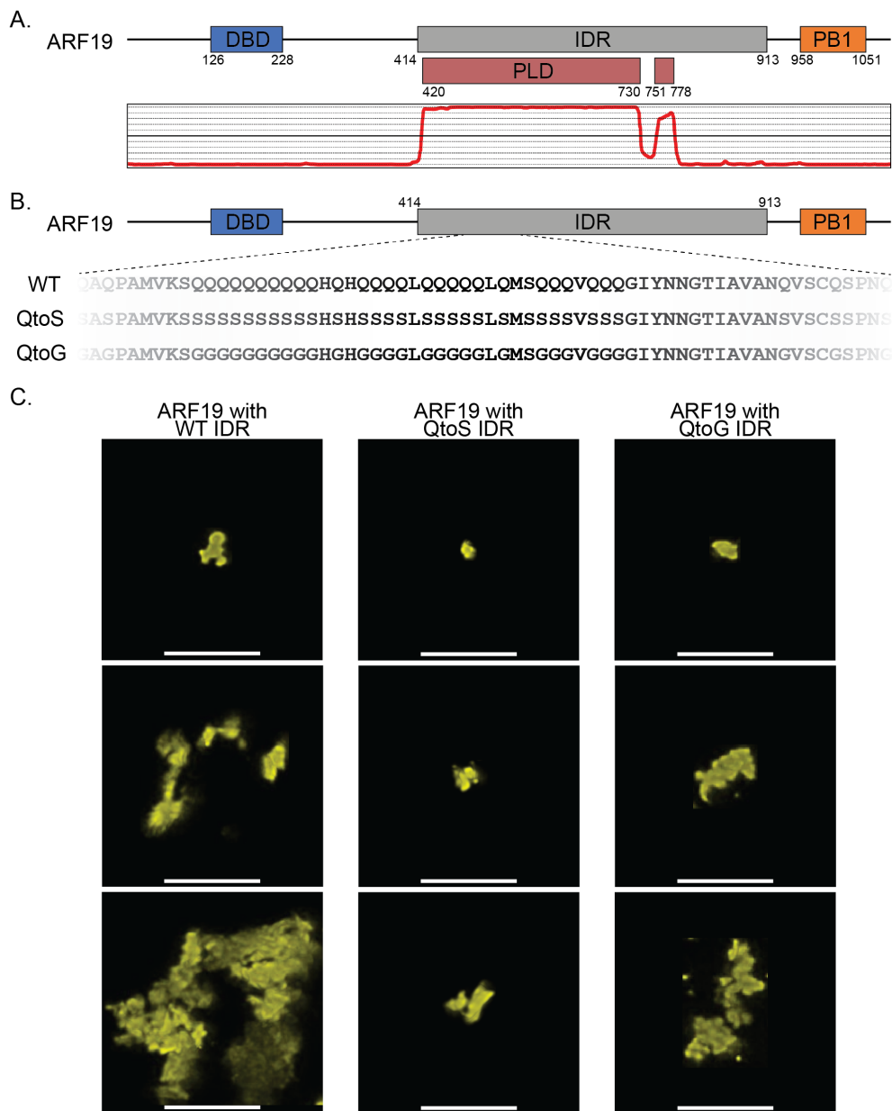
Figure 1. Altering composition of the ARF19 IDR impacts the morphology of ARF19 condensates.
