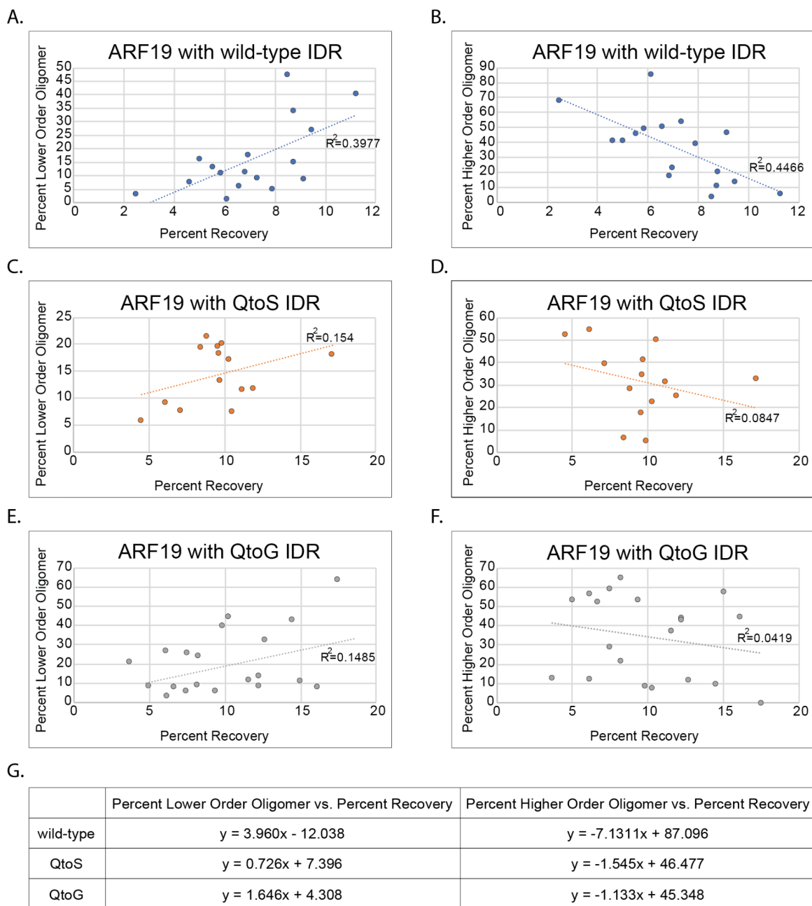
Figure 6. IDR composition-dependent relationship between condensate oligomeric state and fluidity. (A-F) Each point shows N&B and FRAP data for an individual condensate. Panels on the left show the relationship between the percent of lower order oligomers and the fluorescence recovery two minutes post-photobleaching for individual condensates whereas panels on the right show the relationship between higher order oligomers and percent recovery for individual condensates. Dashed lines are linear fit lines. R^2 values are shown near the linear fit lines. N=17 (WT), N=14 (QtoS), and N=20 (QtoG). (G) Equations for linear fit lines shown for each graph.
