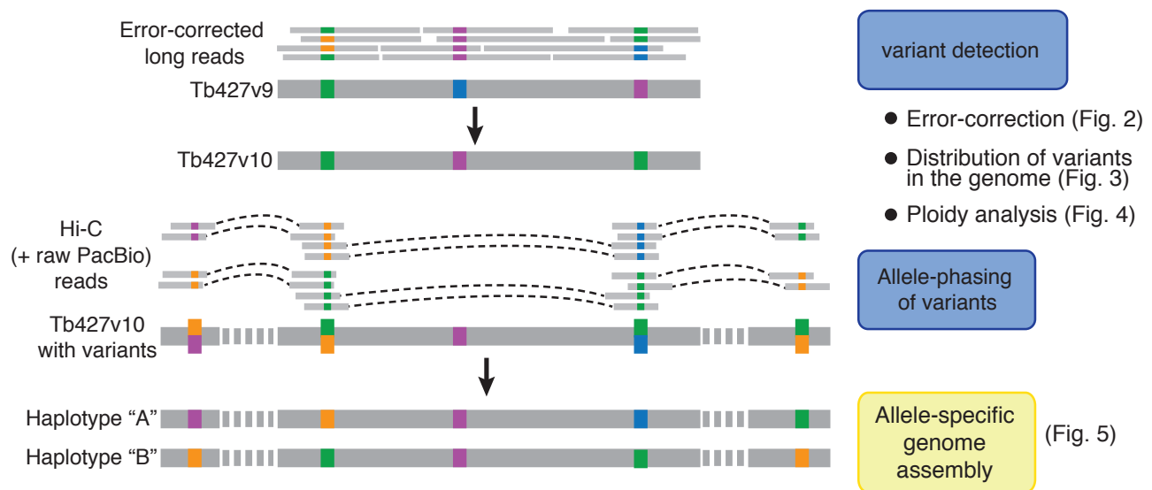
Figure 1. Haplotype phasing procedure. Short-read error-corrected PacBio reads were used to identify variants and fix errors in the T. brucei Lister 427 Tb427v9 genome assembly. Then, the distribution of heterozygous variants along the genome and the ploidy of T. brucei Lister 427 clones was analysed. Finally, Hi-C data and raw PacBio reads were used to link variants and reconstruct the haplotypes of the homologous chromosomes.
