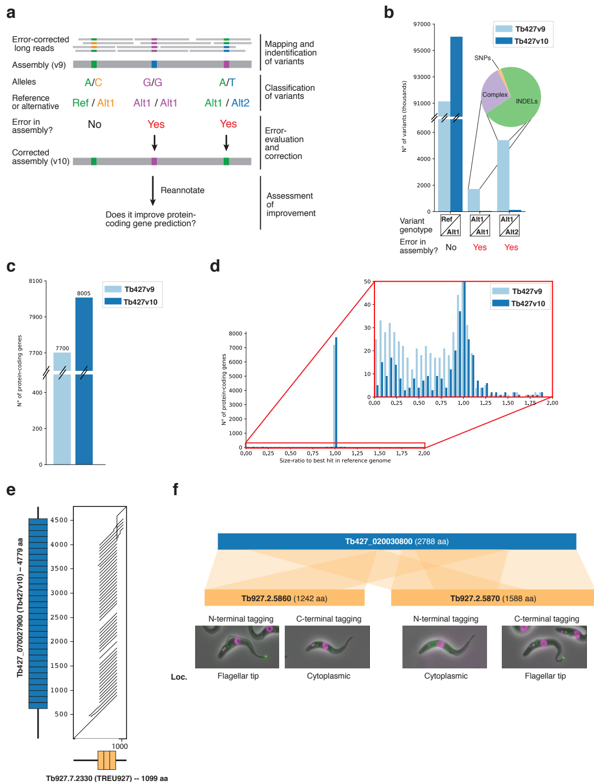
Figure 2. Genome error-correction. a) Error-correction approach. b) Number of variants identified before (Tb427v9) and after error-correction (Tb427v10) of the genome, grouped by variant genotype. The pie chart shows the proportion of SNPs, Complex and INDELs among the error-suggesting variants in Tb427v9. c) Number of protein-coding genes annotated. d) Size-ratio distribution of protein-coding genes compared to the T. brucei TREU927 genome assembly. The right panel is a zoom-in to the region selected in red. e) Alignment dot plot between synthetic orthologs in Tb427v10 (Tb427_070027900) and T. brucei TREU927 (Tb927.7.2330), showing a big repeat-array length difference, illustrated by the number of blue and orange boxes in the gene representations on the axes. f) Alignment of Tb427_020030800 from Tb427v10, to two contiguous protein-coding genes annotated in the T. brucei TREU927 genome assembly (Tb927.2.5860 and Tb927.2.5870), suggesting the gene was wrongly split in the latter assembly. The lower panel shows the subcellular localization (in green) of the N- and C-terminal tagged versions of Tb927.2.5860 and Tb927.2.5870 (data provided by TrypTag.org).
