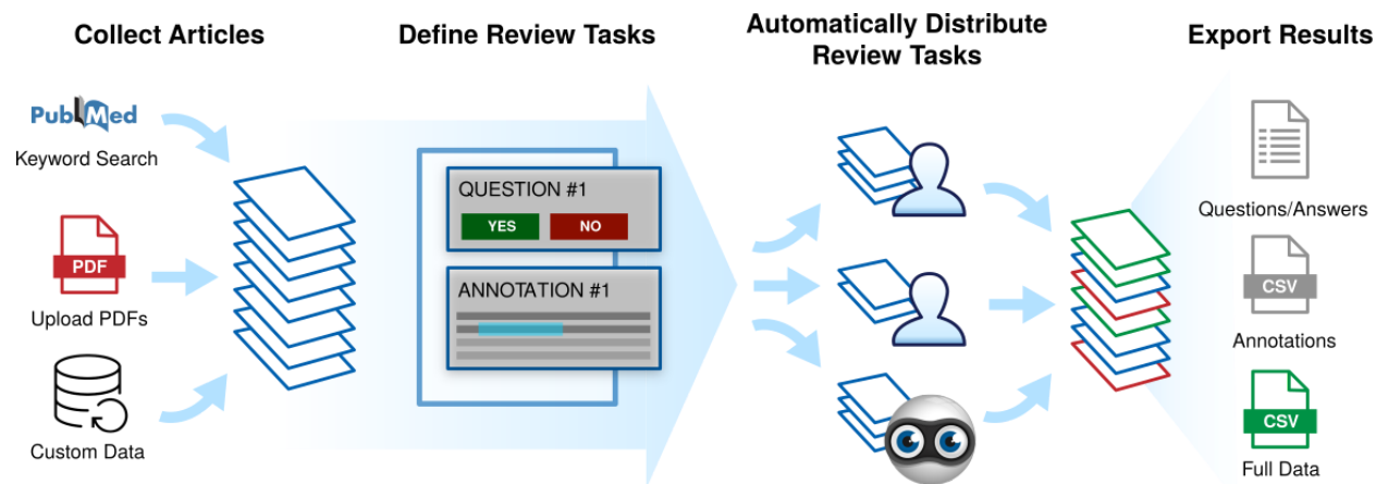
Figure 1. Sysrev projects can be broken into 6 stages from left to right (1) articles are collected to form a data source (2) review tasks or 'labels' are defined (3,4) reviewers are recruited and asked to complete review tasks. Active learning is involved at this stage to prioritize and replicate labelling tasks (5,6) data is exported and analyzed.
