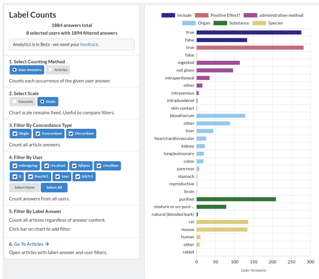
Figure 3 A screenshot of the sysrev label counting tool. A demonstration of this tool is publicly available at https://sysrev.com/o/2/p/21696/analytics/labels . Label counts can be filtered, visualized and updated in real time as a sysrev progresses.
