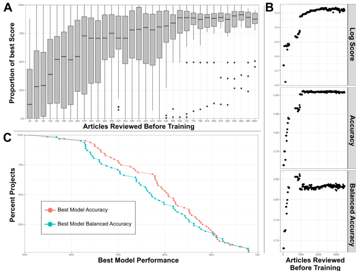
Figure 7. A. Box plots indicate distribution of model performance relative to the worst and best model in a given model's project. Models are bucketed according to the number of articles labeled before model training. Models improve rapidly until 300 articles have been reviewed. B. Accuracy metrics for a large sysrev reviewing insect population changes. Model performance is charted as a function of number of articles used in training, across 3 performance metrics, and evaluated on a consistent holdout set. C. Best model accuracy and balanced accuracy evaluated in 64 sysrevs.
