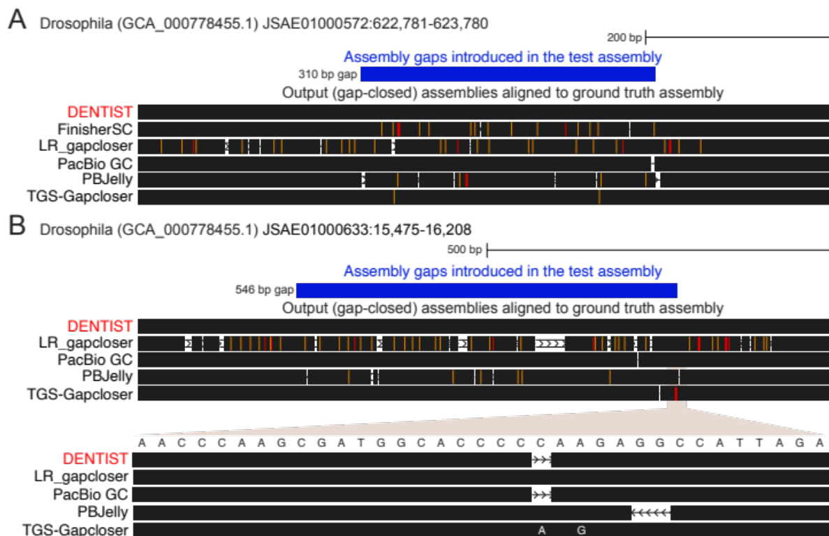
Figure 4: Examples of gaps in the Drosophila assembly that are closed with real PacBio reads.
