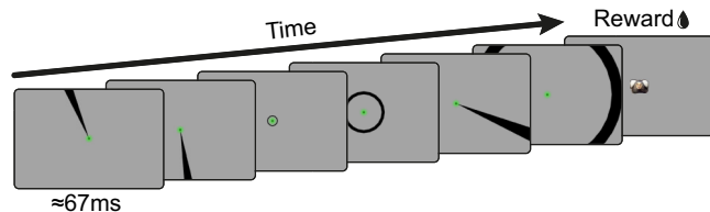
Figure 6. Receptive field mapping task. Annulus and wedge stimuli with sizes and orientations that covered the whole monitor were flashed for 8 frames ( \approx 67 ms) each. The animal was required to maintain fixation throughout the trial and was rewarded at the end. Correct trials were signaled by the appearance of a marmoset face at the center. Typically, nine to ten stimuli were flashed per trial, but only six are shown here for clarity.
