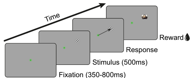
Figure 4. Visual acuity task design. Animals were required to fixate a central fixation point for 350-800 ms. A small Gabor stimulus (0.3 degree, 50% contrast) with variable spatial frequency was presented for 500 ms randomly at one of eight possible locations ( \approx 10.77 degrees eccentricity). After a correct saccade to the target, a picture of a marmoset face was displayed and the animal was rewarded.
