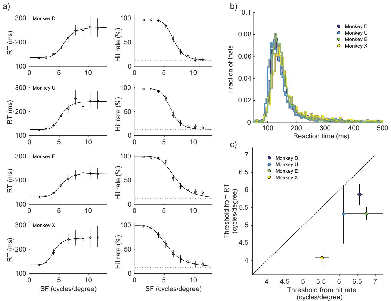
Figure 5. Visual acuity measurements in head-free marmosets. a) Reaction time (RT) and hit rate as a function of stimulus spatial frequency (SF) for each of the four animals. Mean RTs are shown on the left panel and hit rates are shown on the right panel. Error bars indicate 99.9% confidence intervals. In the hit rate plots, dotted lines show expected chance level performance of 12.5%. b) RT distributions, per animal, pooled over all conditions and sessions. c) Comparison of acuity thresholds calculated from RTs and hit rates. Error bars indicate 95% confidence intervals.
