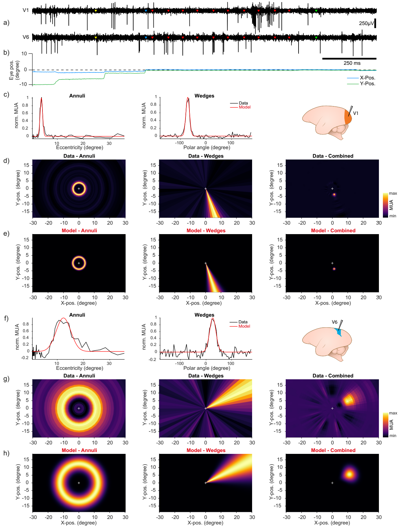
Figure 7. Receptive field mapping results. a) Spiking activity from two example channels simultaneously recorded from cortical areas V1 and V6 in Monkey A. Yellow markers indicate start of the trial. Blue markers indicate fixation onset. Red markers indicate onsets of individual stimuli. Green markers indicate time of reward. b) Corresponding eye trace for example trial. Note fixation onset as indicated by blue markers. c) Multi-unit activity (MUA) profiles and model fits for all presented annuli and wedges from an example recording site in area V1. d) Reverse correlation RF maps across the monitor, from annulus, wedge and combined MUA data. Color indicates normalized multi-unit response. White cross indicates position of fixation point at the center of the monitor. e) RF maps across the monitor, from annulus, wedge and combined model data. f-h) Same as c-e) but from recording site in area V6 in Monkey D.
