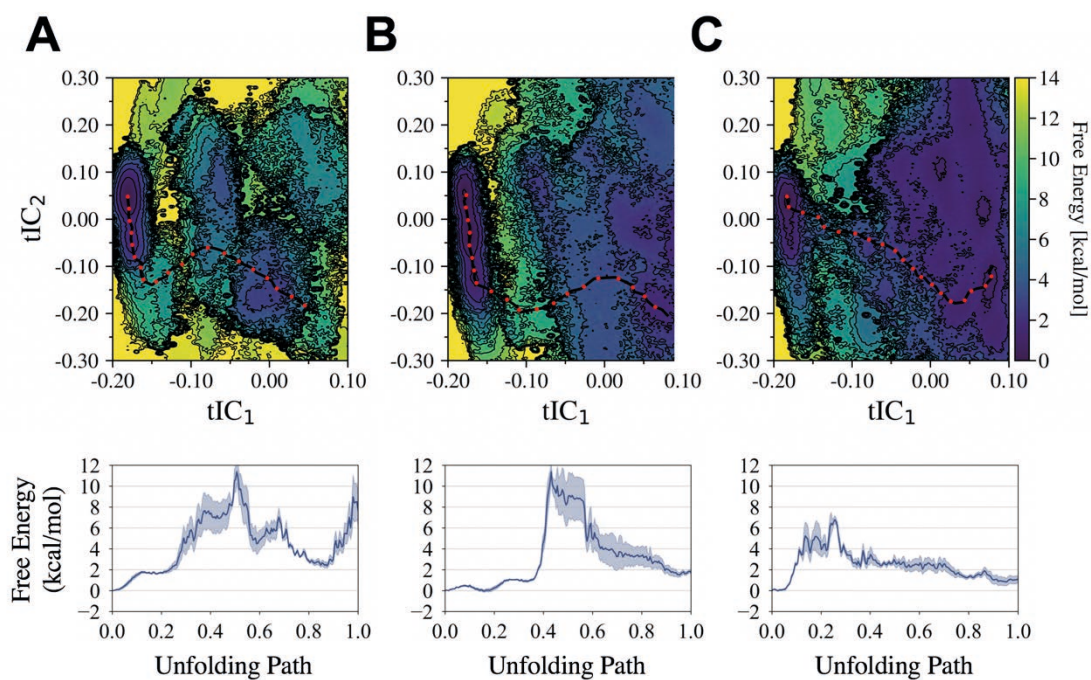
Supplementary Figure 5 An alternate comparison of free energy surfaces projected onto the first ( tIC_1 ) and second ( tIC_2 ) time-structure independent components. We compare (A) a helix in a complete hexamer to (B, C) helices in an incomplete hexamer missing 2 neighboring CA-SP1 monomers, where (B) is a helix between two neighboring helices and (C) is the outer helix (with V362 and A366 exposed to solvent). Each respective minimum free energy path is depicted as a black line with red dots and quantified in each of the bottom plots. In each case, the 6HB is coordinated by IP_6 .
