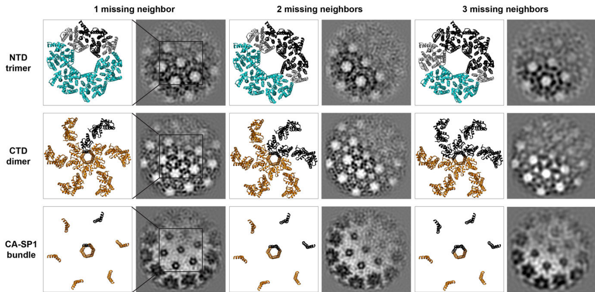
Figure 2 Cryo-EM structures obtained by WMD PCA classification of lattice edge hexamers. Classes with varying numbers of missing neighbors are shown next to corresponding CA_{CTD} and CA_{NTD} atomic models (PDB 5L93) fit as rigid bodies, with a box indicating the region of each class illustrated as an atomic model in each row. Models include the six monomers in the central hexamer, and the 18 surrounding monomers that interact with the central hexamer by either CA_{CTD} dimer or CA_{NTD} trimer interactions. Missing Gag molecules are depicted in black. CA_{NTD} trimers and CA_{CTD} dimers in which all trimer or dimer partners are present are shown in cyan and orange respectively. CA_{NTD} trimer positions which are missing trimer or dimer binding partners are shown in gray.
