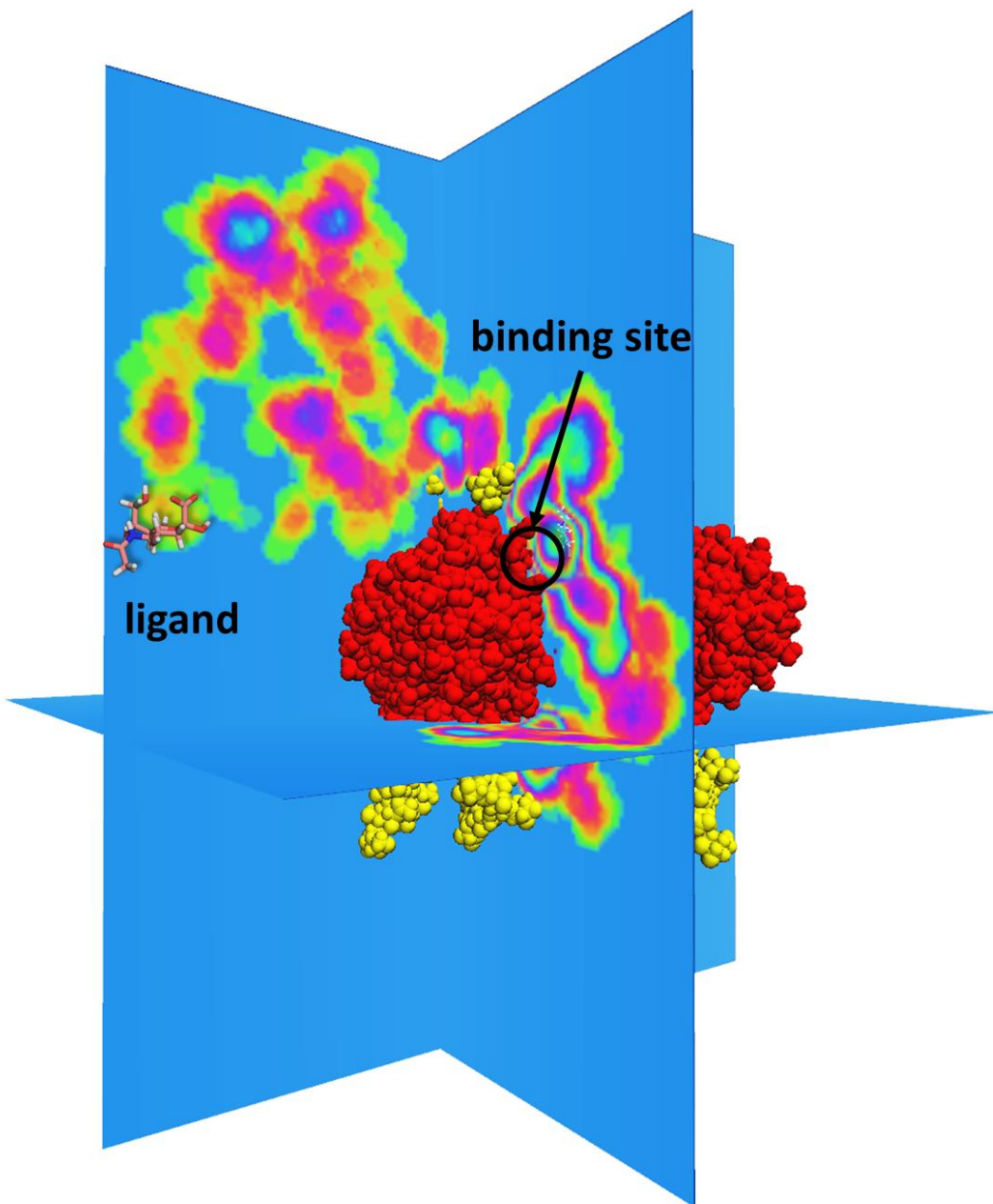
Figure 6. A sample successful trajectory, showing that the ligand explores significant space before finding the binding site. Because of the space explored, it makes sense that a blockage in part of the path won't significantly affect the association rate. Here, the protein is in red and the glycans are in yellow. The blue planes are used for creating subsections of 3D space into 2D space. The colors on the planes indicate how often the ligand has spent in that 2D space, with the lime green inside magenta circles being the most occupied.
