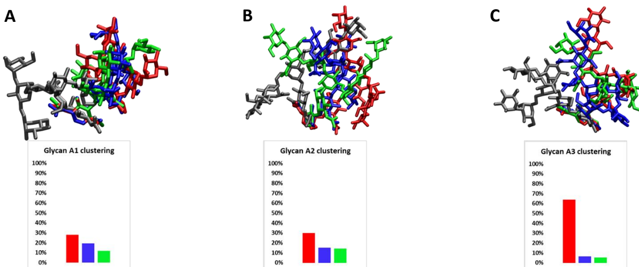
Figure 3. Clustered glycans on monomer A. The glyprot structure is in gray, while the other colors represent clusters from the MD simulations.
