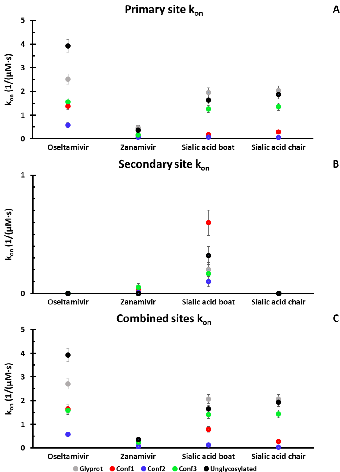
Figure 5. Association rates of each ligand to the primary and secondary sites. Conf1 is the glycan structure from the most populated cluster from the MD simulations. Conf2 is from the second most populated cluster, and conf3 is from the third most populated cluster. The association rates using glycans structures downloaded from Glyprot are shown in gray. The association rates using structures derived from the MD simulations are in bright, colorful shades
