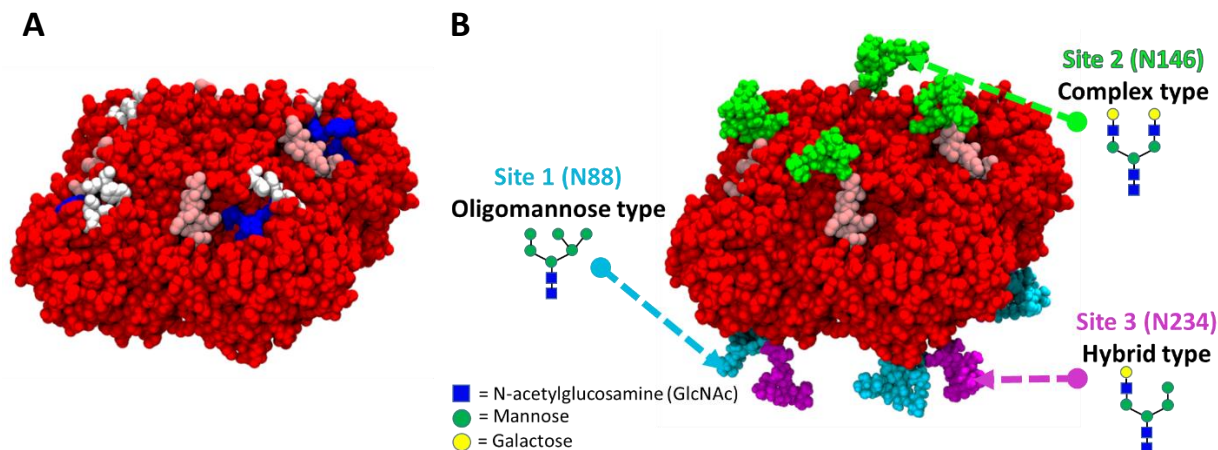
Figure 1. Structure of the NA head. (A) The relation of the binding sites to the 150 loop and each other are shown. The NA protein is in red, the 150-loop is in pink, the primary binding site is in blue, and the secondary binding site in white. (B) The glycan structures and types used in this study are shown in relation to the 150 loop. The glycan on top of each monomer is attached to the 150 loop. Three unique glycan structures and types were used in the simulations. The font color of the glycosylation site refers to the corresponding glycan structure on the protein.
