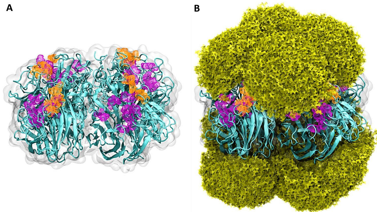
Figure 2. Glycan shielding on NA. (A) Molecular representation of the unglycosylated NA's homotetrameric head showing accessible binding sites. The static structure of NA is in teal. The primary binding sites are in purple, and the secondary binding sites are in orange. (B) Molecular representation of the glycosylated NA's homotetrameric head showing much of its surface area shielded. The static structure of NA is in teal, the primary binding sites are in purple, and the secondary binding sites are in orange. The glycan shield is represented with a yellow cloud of triangles using multiple layered glycan conformations from the MD simulations. A total of 100 frames, using a stride of 10, were selected from the 1000 frames-long trajectory obtained upon concatenation of all the MD simulations.
