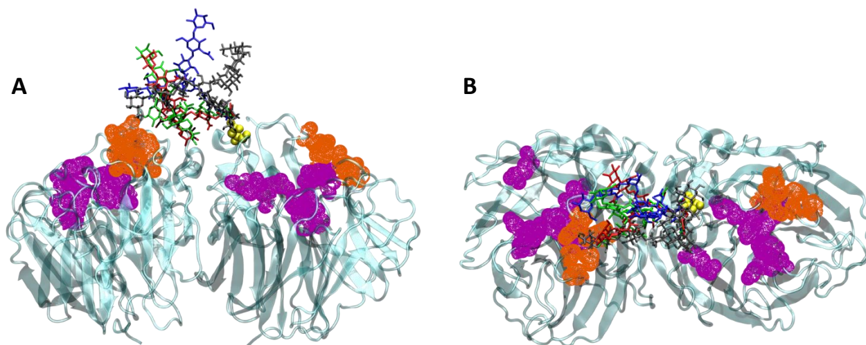
Figure 4. The superposition of each glycan onto the static NA structure shows the conformational variation of the glycans. (A) Side view and (B) top view of the glycosylated NA model with MD-derived glycan conformations. For ease of viewing, only two monomers are shown here, with the glycans only coming from the monomer on the right in panel (A) and panel (B). The yellow glycosylation site N88 and the attached glycans reside in the same monomer. The glycans bend away from the binding sites on their monomer towards the binding sites on the neighboring monomer. This is seen for each monomer. The primary binding sites are in purple and the secondary binding sites are in orange. The linkage between the glycans and the protein is in yellow. The NA structure is in teal.
