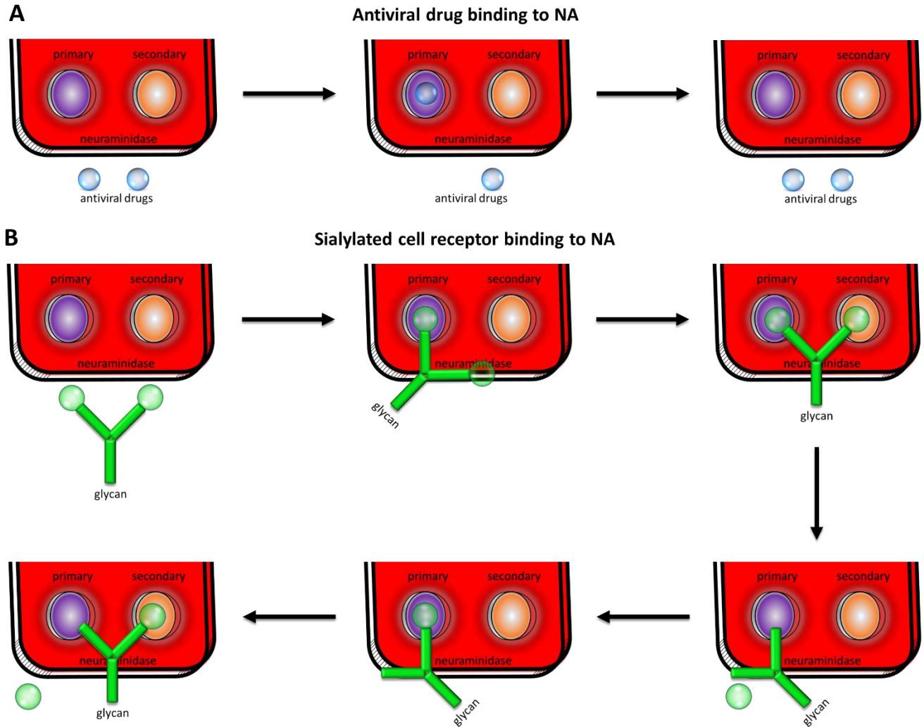
Figure 7. Ligand binding mechanisms to neuraminidase for monovalent binders (A) and multivalent binders (B). A free monovalent binder will associate to the primary site over the secondary site (A). This monovalent binder will release from the primary site before a second monovalent binder will associate to the secondary site. Glycans, with their sialic acid tips, are an example of a multivalent binder (B). Similar to the monovalent binders, the first multivalent binding event will occur to the primary site. Next, the second sialic acid tip binds to the secondary site. With both sites bound, the sialic acid in the primary site is cleaved and released. The sialic acid bound in the secondary site is then transferred to the primary site. Finally, the second sialic acid is cleaved and released, and the enzymatic cycle is complete.
