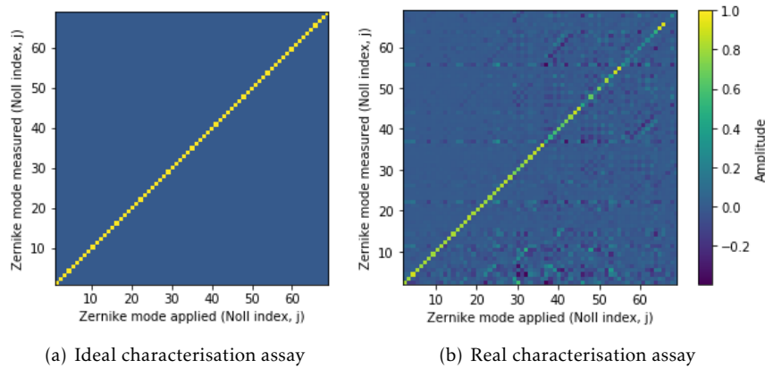
Figure 4: (a) An ideal characterisation assay, measuring the recreation accuracy of 68 Zernike modes with applied amplitude of 1 for each (b) A realistic characterisation assay obtained from a calibrated Alpao-69 actuator deformable mirror, measuring the recreation accuracy of 68 Zernike modes with applied amplitude of 1 for each
