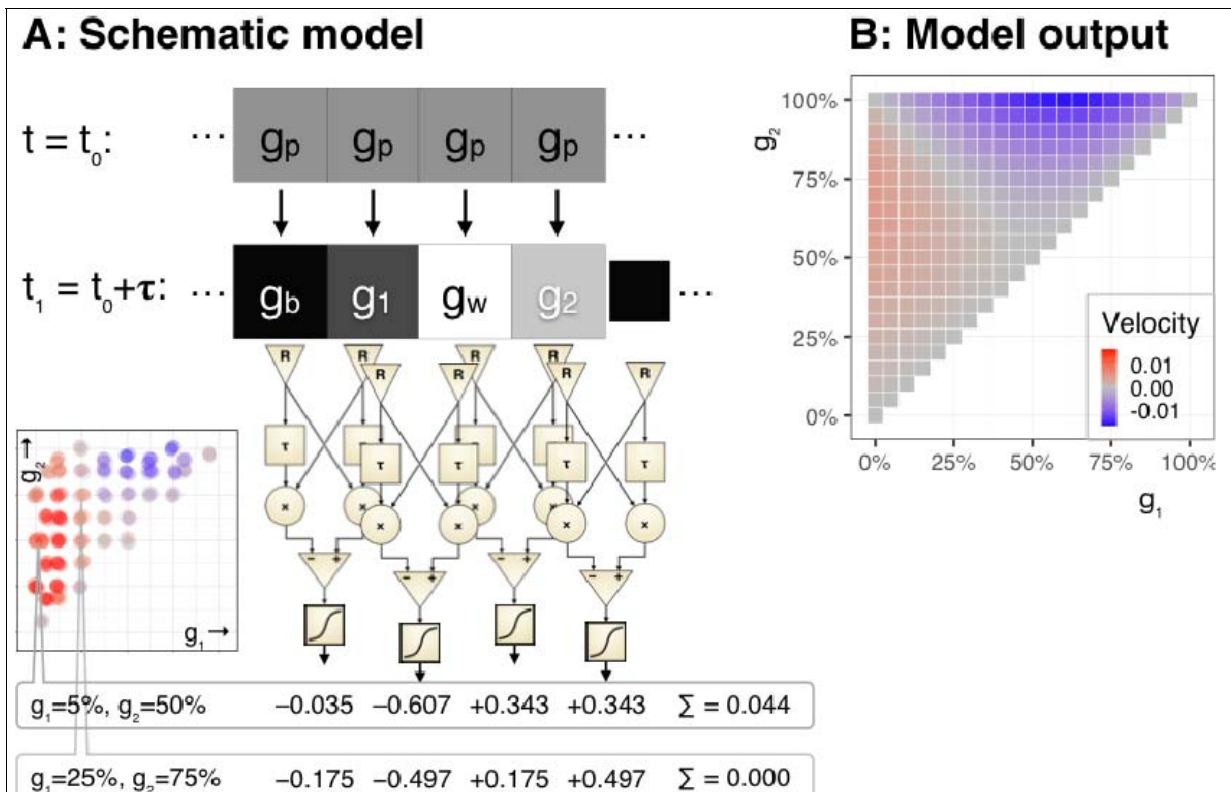
Fig. 2 – Model, first approximation. A. On top, a sequence of grey squares turns into the Snake sequence below. That sequence is the input to an array of motion detectors (cf. Fig. 1), whose output is calculated for two example combinations of (g_1, g_2) . The positions of these (g_1, g_2) are indicated on a psychophysical data map (bottom left) which we reported previously (Atala-Gerard and Bach 2017), showing two parameter regions which result in opposite illusory motion direction. The first (g_1, g_2) pair is from the region of strongest observed illusion, and indeed the average of the four outputs yields a non-negative value. The second (g_1, g_2) pair (25%, 75%) is from the “valley” between the two regions (the diagonal), and for symmetry reasons yields a zero net motion output. B. Net motion output example for all (g_1, g_2) pairs. It bears a qualitative similarity to the psychophysical findings (shown in figure part A, bottom left): There is a motion maximum near the expected region ( \approx 5\% , 50%) and, indeed, the model predicts an inverse direction near the region where this was experimentally observed (top right).
