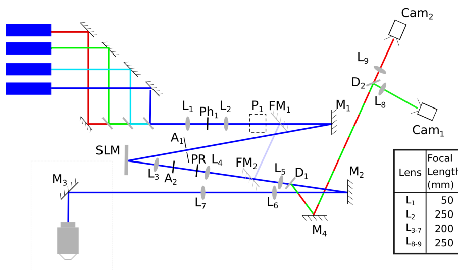
Fig. 2. A schematic of the cryoSIM microscope, with lenses (L), apertures (A), mirrors (M), pinholes (Ph), dichroics (D), periscope (P), polarisation rotator (PR), and cameras (Cam) shown. The four lasers have wavelengths of 405, 488 and 647 nm (Omicron DeepStar lasers) and 561 nm (Cobolt Sapphire laser) were combined and passed through the telescope L 1 and L 2 with a pinhole (Ph 1 ) at its focus to clean up the beam profiles. The beam was reflected reflected towards the SLM by M 1 , through an aperture A 1 . Light reflected from the SLM was refocused by L 3 to aperture A 2 which removed high diffraction orders generated by the SLM. The polarisation was rotated by the PR and the telescope formed by L 4 and L 5 reimaged the diffracted spots onto M 2 , after L 5 the excitation light passed through the dichroic D 1 . The beam continued through telescope L 6 and L 7 via M 3 to the back-pupil of a 100× 0.9 NA air objective and focused into the sample. The fluorescence emission was collected by the objective and reflected from M 3 , passed back through L 7 and L 6 , was reflected M 2 to dichroic D 1 , where the fluorescence emission was reflected off M 4 to the dichroic D 2 . This dichroic split the emitted light between two cameras, Cam 1 and Cam 2 , via imaging lenses L 8 and L 9 . The dotted box in the bottom left hand side was at 90° to the plane of the rest of the diagram, so while most of the optics are in the horizontal plane, the objective is vertical and pointing downwards. There are two flip mirrors FM 1 and FM 2 which bypass the SLM to allow widefield illumination. Lens focal lengths are shown in the table.
