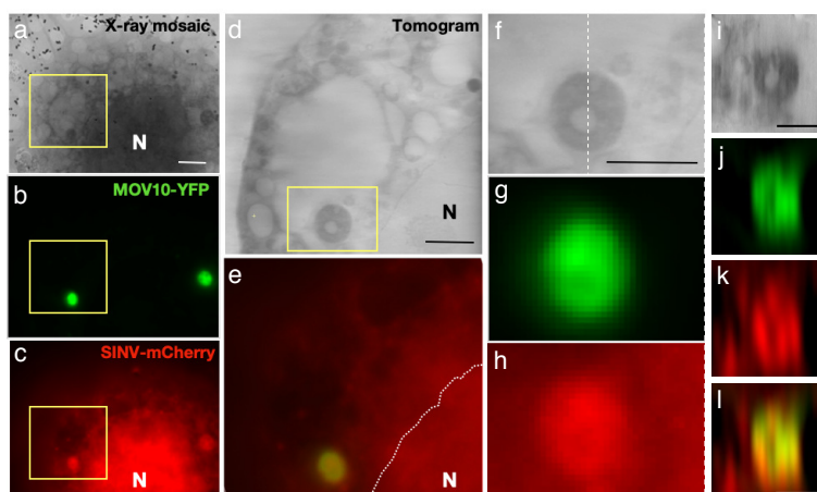
Fig. 7. Correlated cryoSIM and X-ray tomogram
