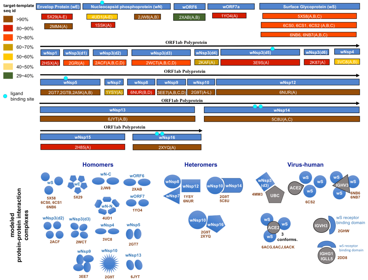
Figure 1. Structural genomics and interactomics road map. Shown are the individual proteins and protein complexes that were targeted for structural characterization together with PDB ID of their templates from Protein Data Bank (PDB).
