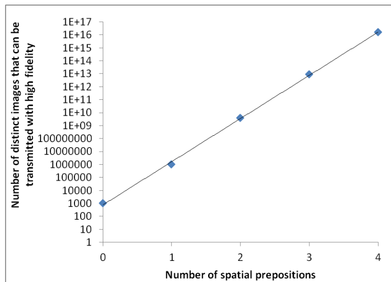
Figure 2. The graph shows the number of distinct images that can be conveyed with high fidelity in a communication system with 1,000 nouns as a function of the number of spatial prepositions.
