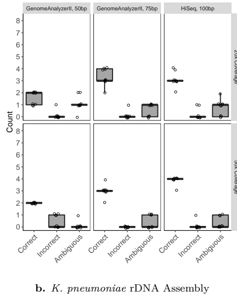
Figure 6: Comparison of de fere novo assemblies of simulated reads generated by pIRS. In most cases, increasing coverage depth and read length resulted in fewer misassemblies. Assemblies were scored using score ; the y axis reflects the total number of rDNAs in the genome (7 and 8 rDNAs, for E. coli and K. pneumoniae respectively). The (n=9) assemblies shown for each genome are the result of differently seeded read simulations.
