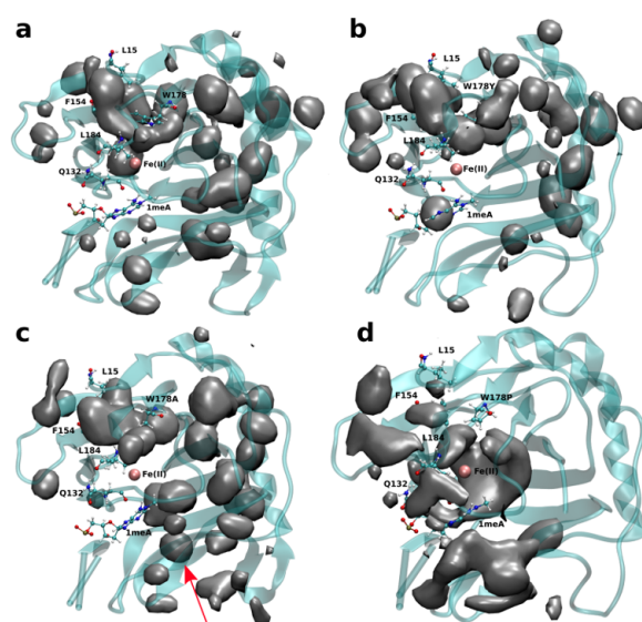
Figure 2: 3D density map representing the O 2 molecule occupancy in a) WT, b) W178Y, c) W178A, d) W178P. The O 2 molecules diffuse through the blue tunnel for wild type and W178Y. W178A reveals a new pathway beside the blue tunnel indicated by a red arrow. O 2 molecules are delivered through the blue tunnel and exhibit long residence times around Fe(II) in the W178P mutant. The isovalue for all density maps is 0.006.
