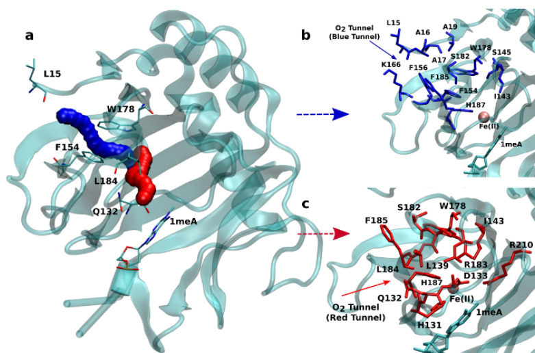
Figure 1: a) Two main tunnels obtained with CAVER for the crystal structure of AlkB. Residues that define the blue (b) and red (c) tunnels.
