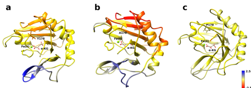
Figure 3: RMSF difference between wild type and mutants along the sampled trajectories for (a) W178Y, (b) W178A and (c) W178P. Residues in blue(red) denote larger(smaller) fluctuations in the mutant structures compared to the wild type.
