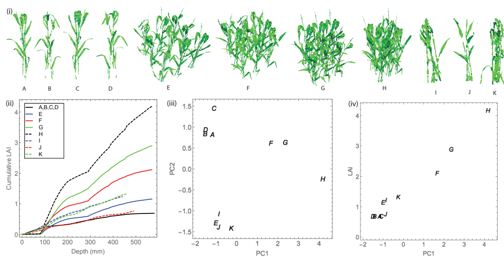
Figure 4: Relationship between the two-state Markov model and canopy physiology: (i) Reconstructed plants (A-K), (ii) cumulative leaf area index as a function of depth (bottom left), (iii) principal component analysis of fitted parameters, and (iv) relationship between the first principal component and LAI. Images of original plant ( A ); original plant rotated 90^\circ ( B ), 180^\circ ( C ), and 270^\circ ( D ); original plant randomly rotated and positioned at distances 200mm ( E ), 150mm ( F ), 125mm ( G ), and 100mm ( H ); replica of a plant from the same line ( I ); plants from two different lines ( J and K ). For more detailed description of the lines used and information on the trial see Burgess et al. (2015).
