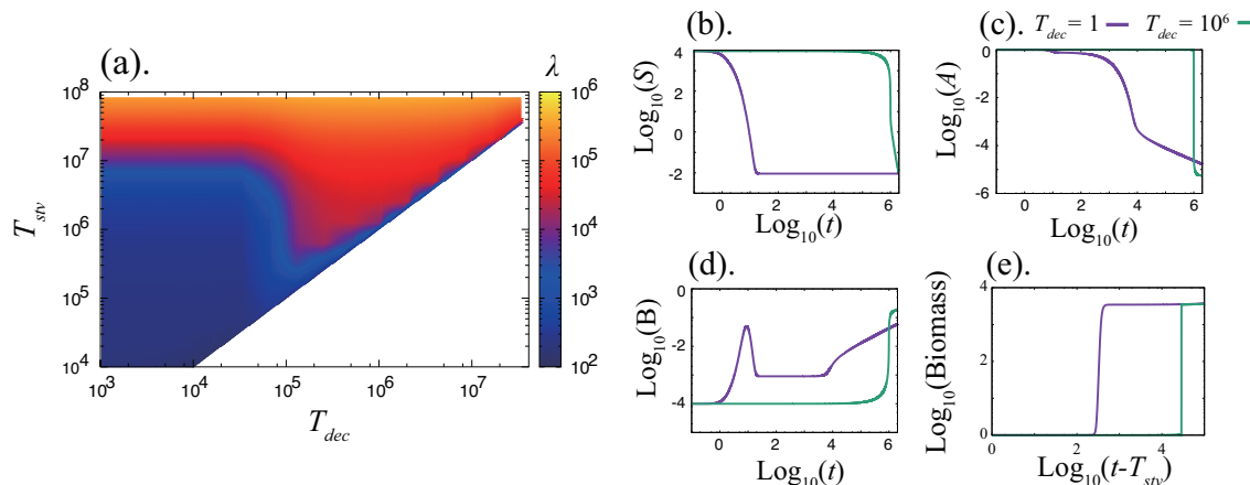
FIG. 3. (a) Dependence of lag time \lambda on the time required to decrease the substrate T_{dec} and starvation time T_{stv} . (b-d) Time series of starvation for different T_{dec} ( T_{dec} = 10^6 (green) and T_{dec} = 1.0 (purple)) values, the internal concentrations of substrate S (b), component A (c), and component B (d). (e) Time series of biomass during resurrection. The same parameter values as indicated in Fig.2 were adopted. The batch culture model (which is used to compute a bacterial growth curve) was adopted to compute the time series of biomass accumulation(e). Time series of \mu is shown in Fig.S3.
