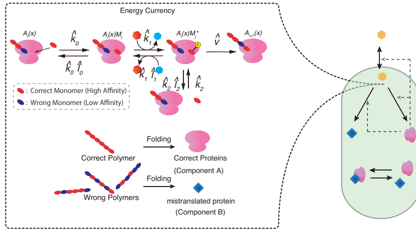
FIG. 7. Schematic representation of a polymer elongation system with kinetic proofreading. The reactions other than the synthesis part ( F_A(S)A and F_B(S)A ) are identical to those of the original model (2).
