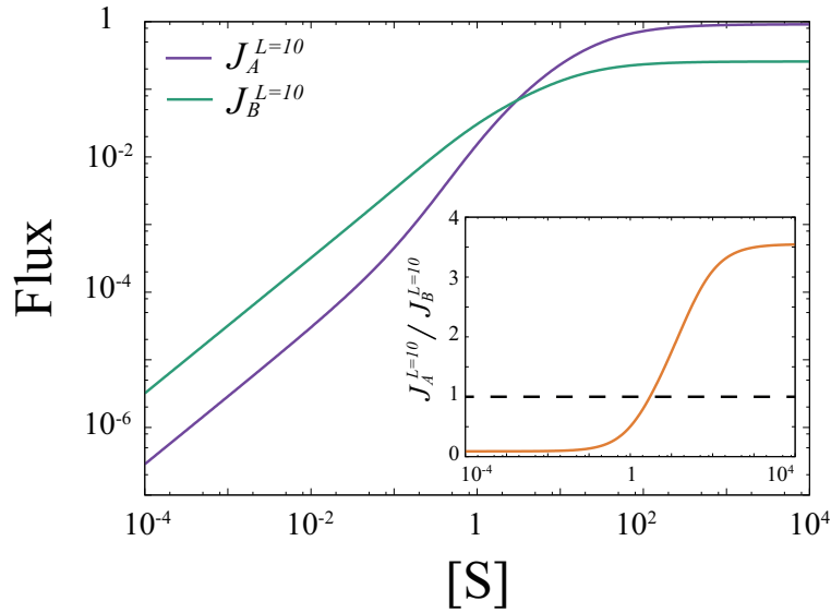
FIG. 8. J_A^{L=10} and J_B^{L=10} are plotted against the substrate concentration [S] . The ratio of J_A^{L=10} to J_B^{L=10} is also plotted in the inset of the figure. Parameters for the polymer elongation part are set to be \hat{v} = 0.1 , \rho_C = 1.0 , \rho_D = 10.0 , \hat{k}_0 = 10^5 , \hat{k}_1 = 10^2 , \hat{k}_2 = 10.0 , \hat{l}_0 = \hat{l}_1 = \exp(-1) , \hat{l}_2 = \exp(1) , K_a = 10.0 , K_S = 1.0 , [M]_{\max} = 1.0 , and [A_0] = 1.0 .
