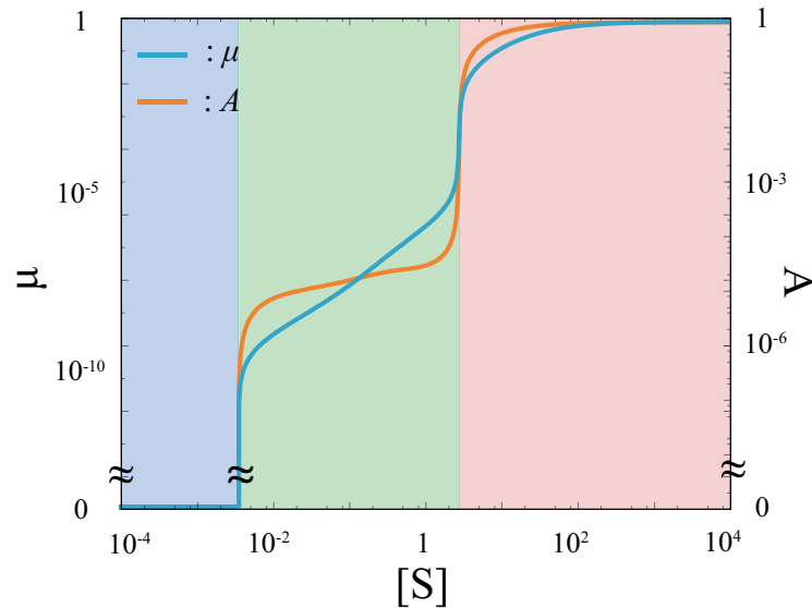
FIG. 9. Steady growth rate of the model with polymerization and kinetic proofreading. J_A^{L=10} and J_B^{L=10} are adopted for the synthetic reaction rate of components A and B. Parameters for J_A^{L=10} and J_B^{L=10} are identical to those in Fig. 8, and others are set to be the same.
