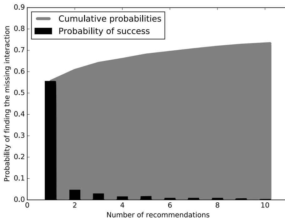
Figure 2: After removing a prey from a predator, we ask the KNN algorithms with Tanimoto measure to make 10 recommendations (from best to worst). The figure shows how many recommendations are required to retrieve the missing interaction. Most retrieved interactions are found with the first attempt. This data was generated with K = 7 and w_t = 0 .
