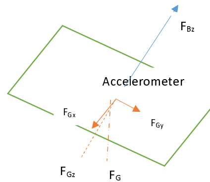
Accelerometer plane at an incline with Earth's Surface
