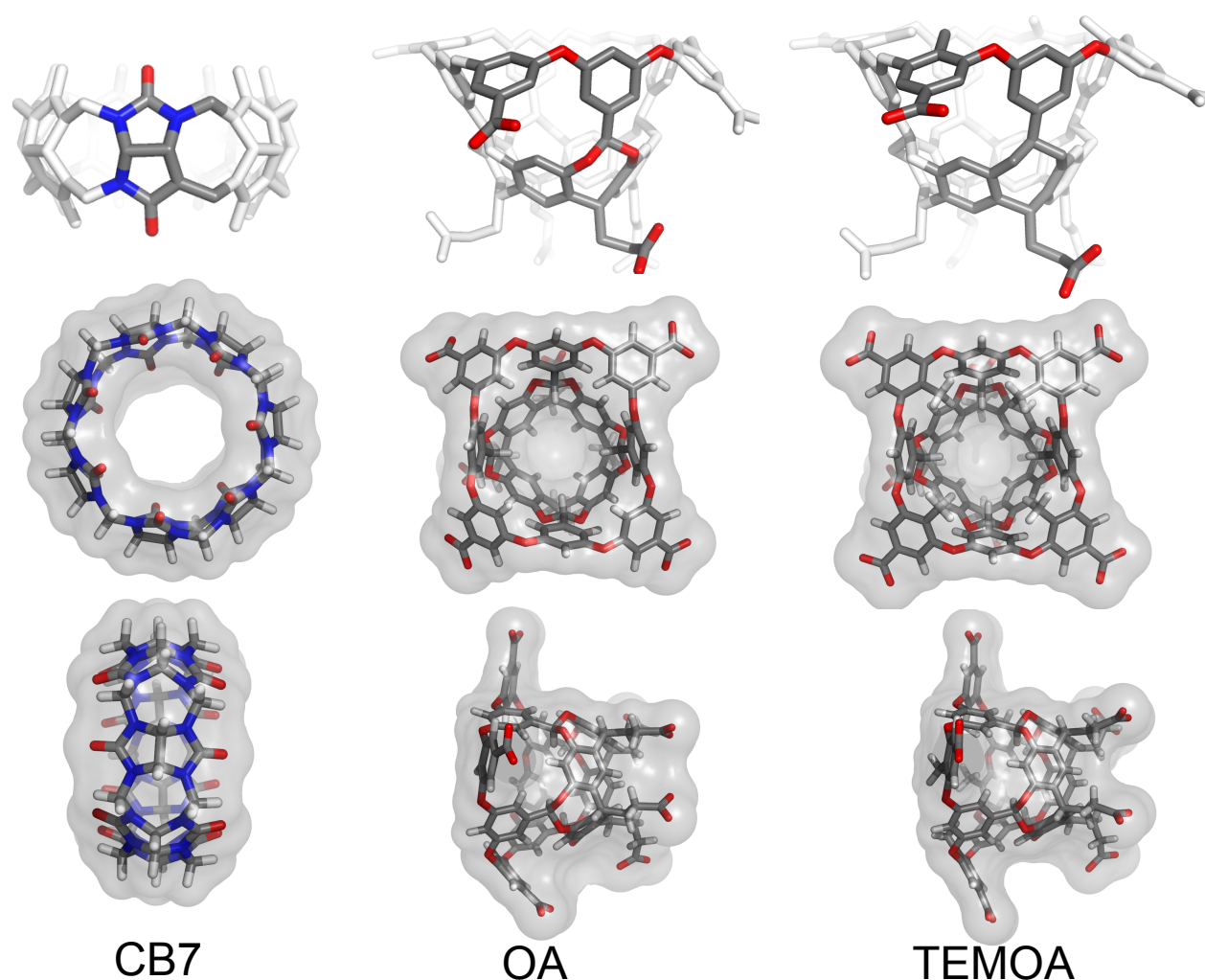
FIG. 1. OA, TEMOA, and CB7 hosts. Shown are the hosts which are the focus of our host-guest benchmark sets – two variants of the octa-acid GDCC, and CB7, a cucurbituril. Guest structures are available in the supplemental material.
